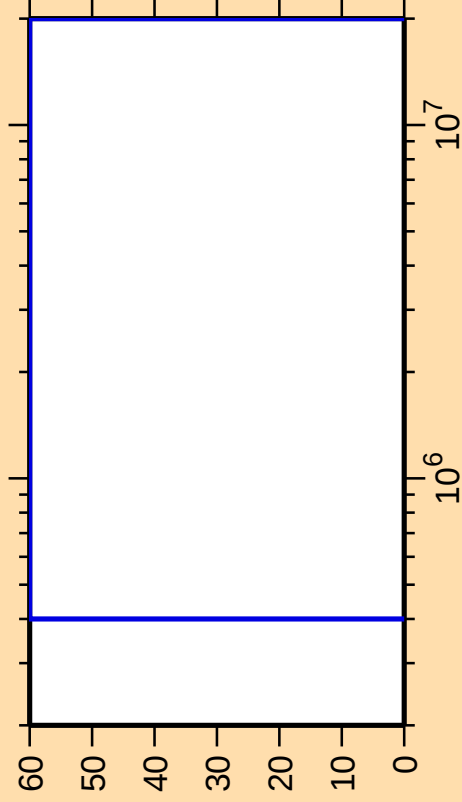
\Delta\sigma/\sigma vs. E for ^{161}\text{Ta}(n,\alpha)
