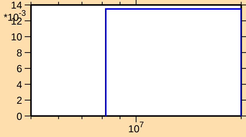
\sigma vs. E for ^{161}\text{Ta}(n,2n)
