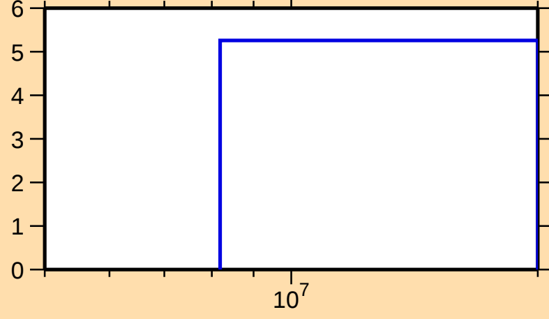
\Delta\sigma/\sigma vs. E for ^{161}\text{Ta}(n,\text{el.})
