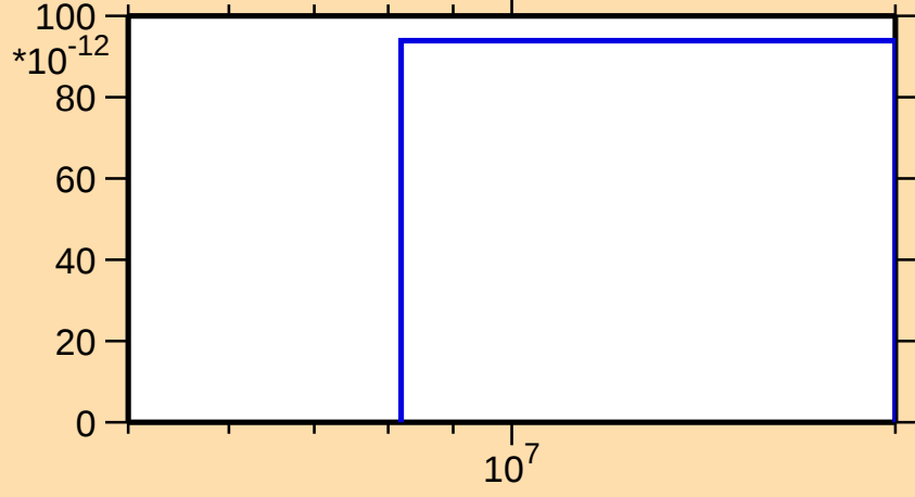
\sigma vs. E for ^{161}\text{Ta}(n,nt)
