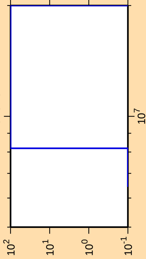
\Delta\sigma/\sigma vs. E for ^{161}\text{Ta}(n,\text{pd})
