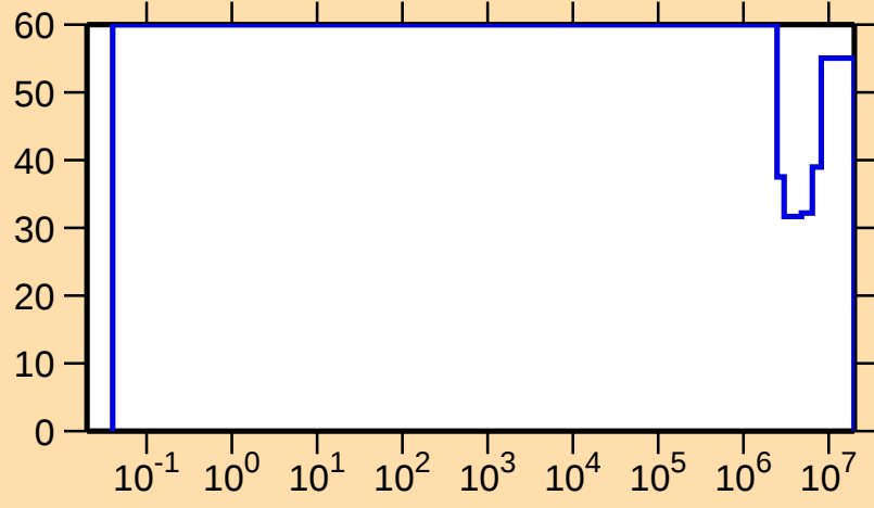
\Delta\sigma/\sigma vs. E for ^{161}\text{Ta}(n,p)
