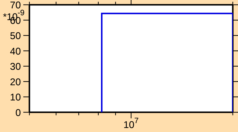
\sigma vs. E for ^{161}\text{Ta}(n,\text{nd})
