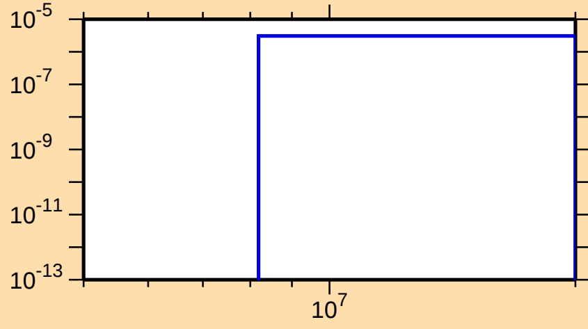
\sigma vs. E for ^{161}\text{Ta}(n,\text{pd})
