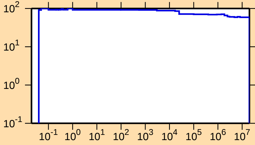
\Delta\sigma/\sigma vs. E for ^{161}\text{Ta}(n,\gamma)
