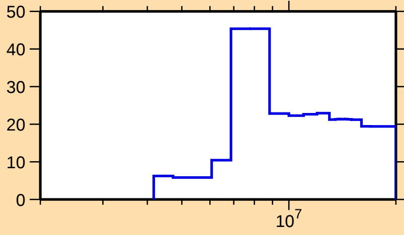
\Delta\sigma/\sigma vs. E for ^{187}\text{Ta}(n,n\text{cont.})
