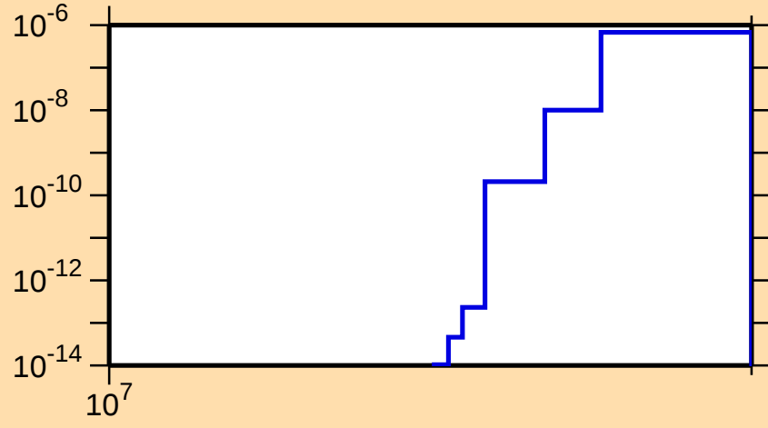
\sigma vs. E for ^{187}\text{Ta}(n,\text{nd})
