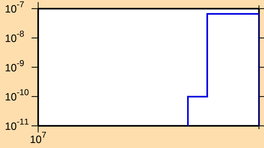
\sigma vs. E for ^{187}\text{Ta}(n,2np)
