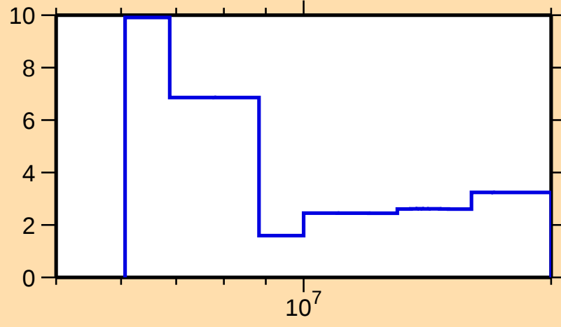
\Delta\sigma/\sigma vs. E for ^{187}\text{Ta}(n,\text{tot.})
