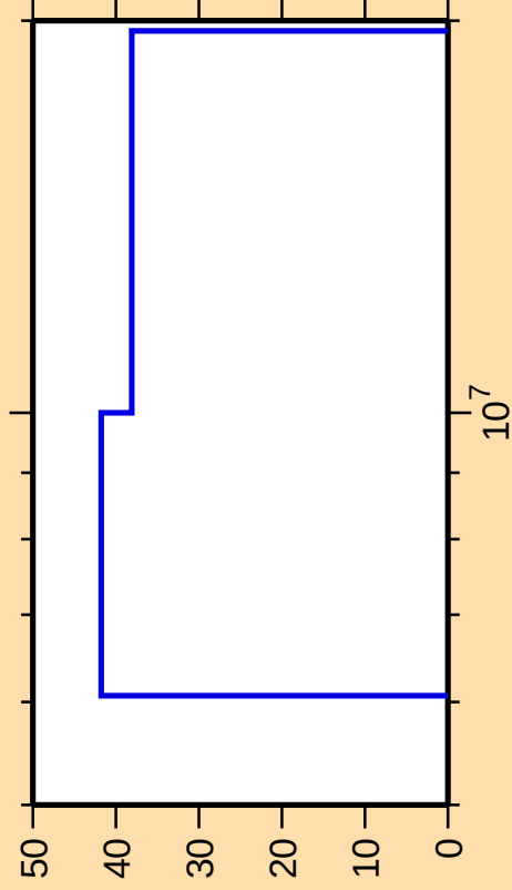
\Delta\sigma/\sigma vs. E for ^{187}\text{Ta}(n,p)
