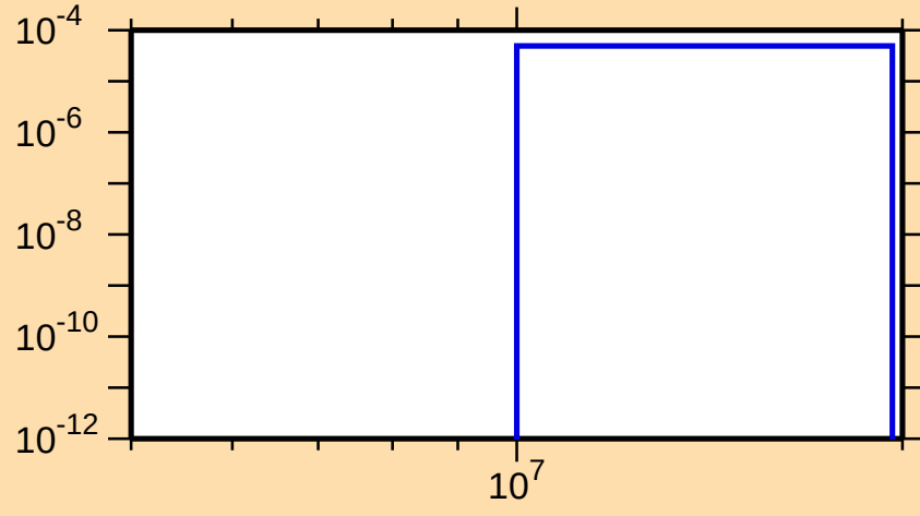
\sigma vs. E for ^{187}\text{Ta}(n,np)
