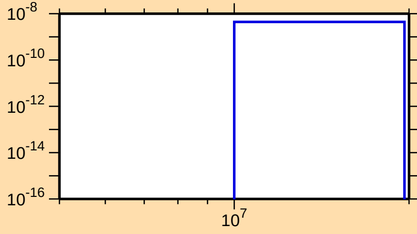
\sigma vs. E for ^{187}\text{Ta}(n,2n\alpha)
