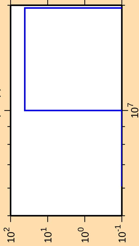
\Delta\sigma/\sigma vs. E for ^{187}\text{Ta}(n,np)
