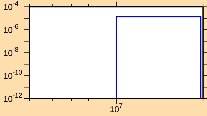
\sigma vs. E for ^{187}\text{Ta}(n,t)
