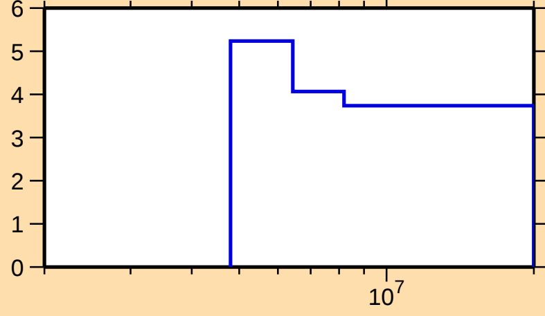
\Delta\sigma/\sigma vs. E for ^{187}\text{Ta}(n,\text{nonel.})
