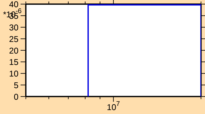
\sigma vs. E for ^{187}\text{Ta}(n,np)
