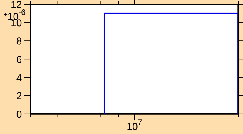
\sigma vs. E for ^{187}\text{Ta}(n,t)
