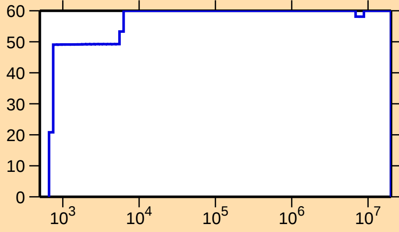
\Delta\sigma/\sigma vs. E for ^{127}\text{Te}(n,\gamma)
