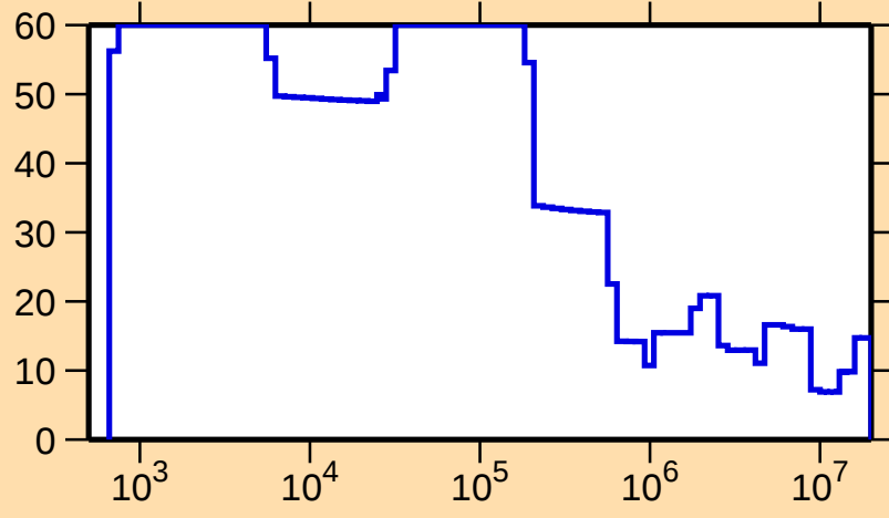
\Delta\sigma/\sigma vs. E for ^{127}\text{Te}(n,\text{el.})
