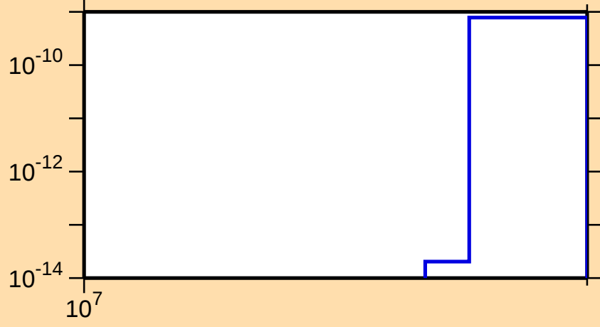
\sigma vs. E for ^{127}\text{Te}(n,\text{nt})
