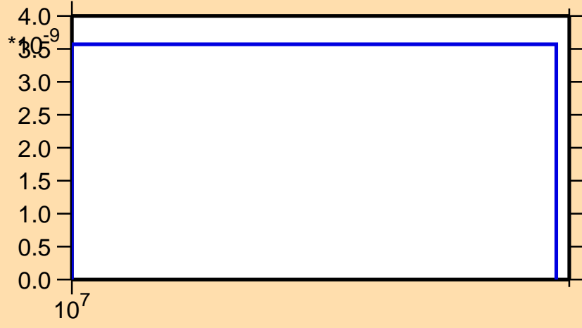
\sigma vs. E for ^{127}\text{Te}(n,2n\alpha)
