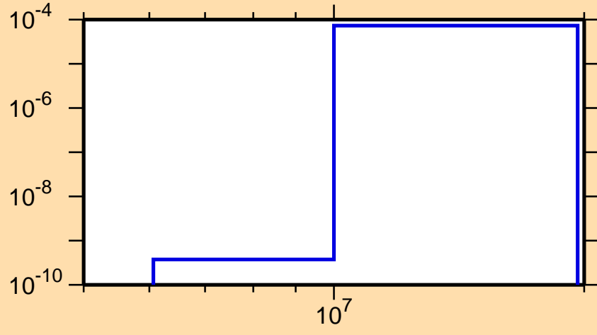
\sigma vs. E for ^{127}\text{Te}(n,n\alpha)
