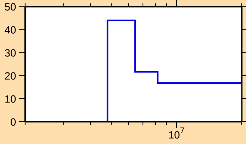
\Delta\sigma/\sigma vs. E for ^{127}\text{Te}(n,2n)
