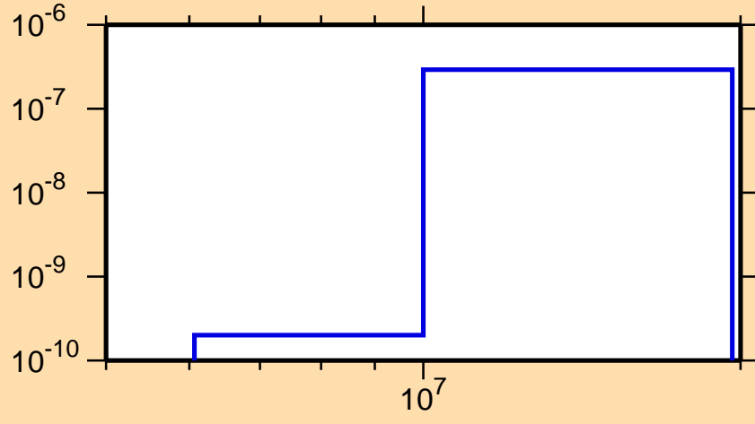
\sigma vs. E for ^{210}\text{Tl}(n,2n\alpha)
