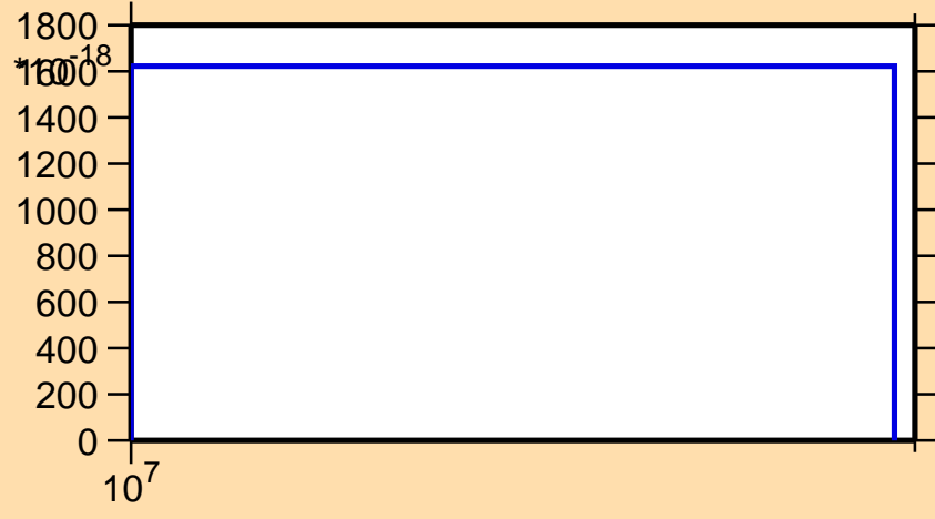
\sigma vs. E for ^{210}\text{Tl} (mt 42)
