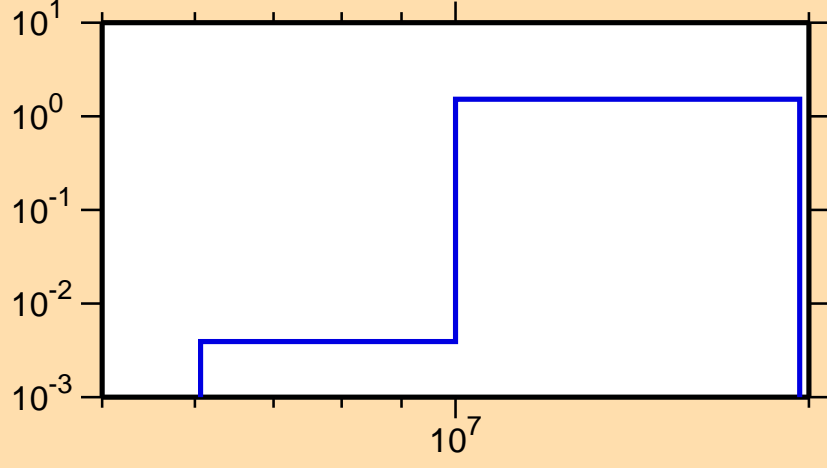
\sigma vs. E for ^{210}\text{Tl}(n,3n)
