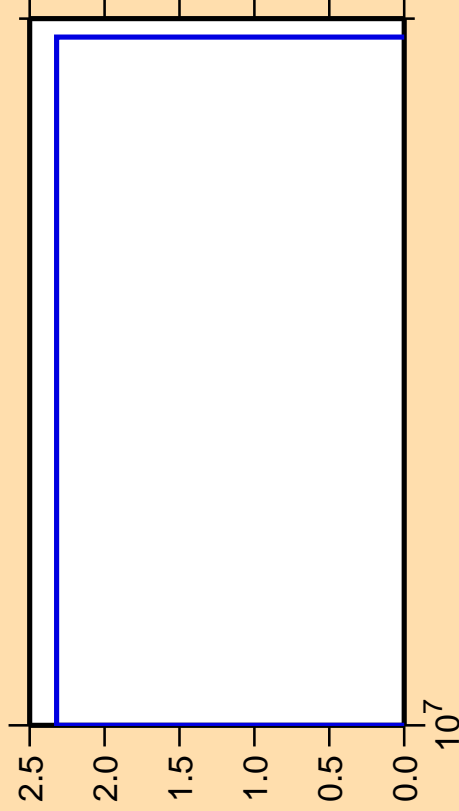
\Delta\sigma/\sigma vs. E for ^{210}\text{Tl} (mt 11)
