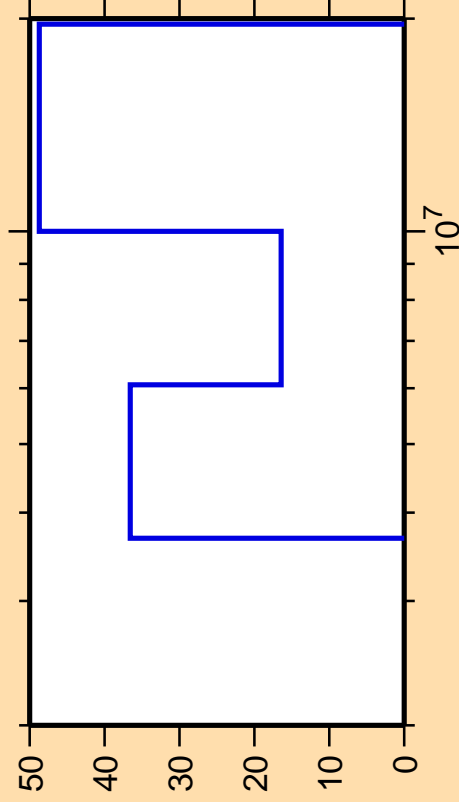
\Delta\sigma/\sigma vs. E for ^{210}\text{Tl}(n,2n)
