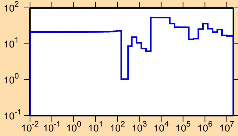
\Delta\sigma/\sigma vs. E for ^{210}\text{Tl}(n,\text{el.})
