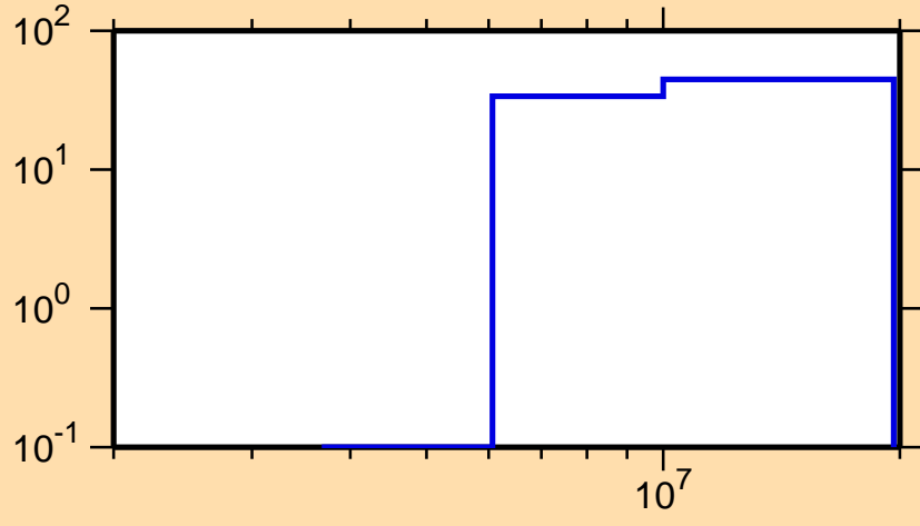
\Delta\sigma/\sigma vs. E for ^{210}\text{Tl}(n,p)
