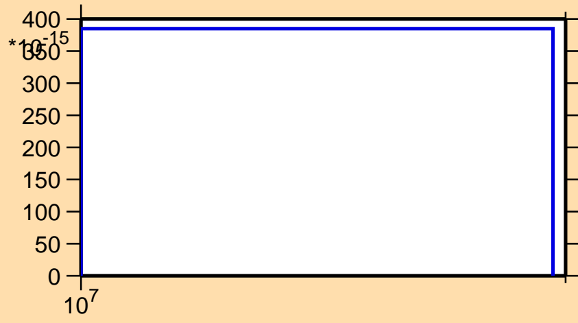
\sigma vs. E for ^{210}\text{Tl} (mt 11)
