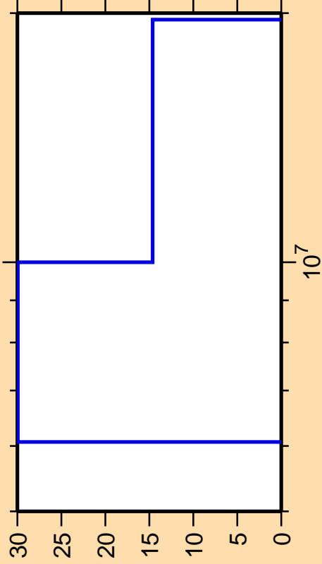
\Delta\sigma/\sigma vs. E for ^{210}\text{Tl}(n,3n)
