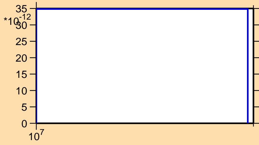
\sigma vs. E for ^{210}\text{Tl}(n,3n\alpha)
