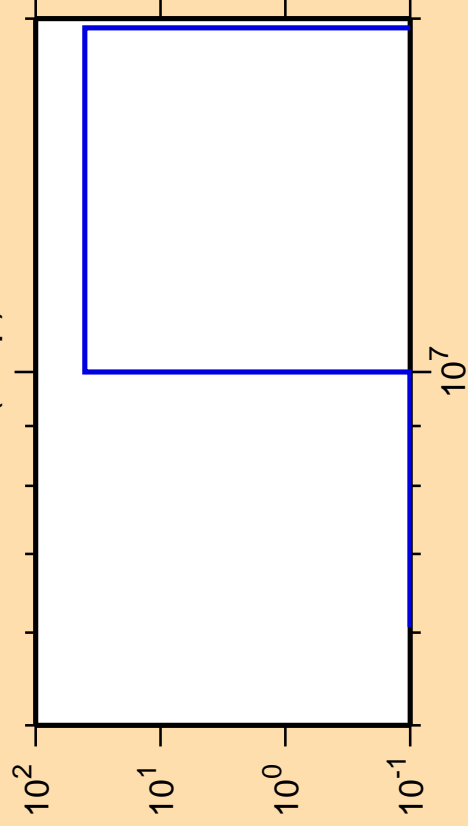
\Delta\sigma/\sigma vs. E for ^{210}\text{Tl}(n,np)
