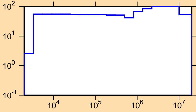
\Delta\sigma/\sigma vs. E for ^{210}\text{Tl}(n,\gamma)
