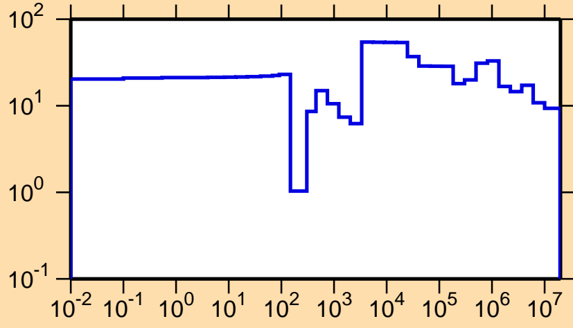
\Delta\sigma/\sigma vs. E for ^{210}\text{Tl}(n,\text{tot.})
