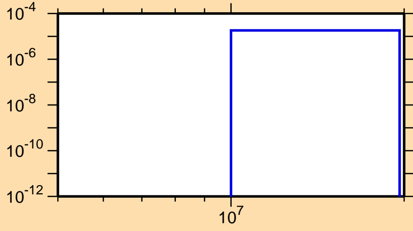
\sigma vs. E for ^{210}\text{Tl}(n,np)
