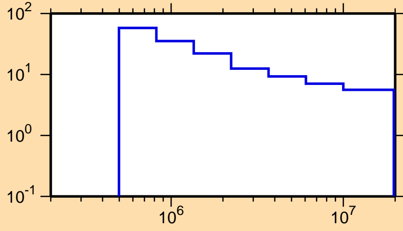
\Delta\sigma/\sigma vs. E for ^{210}\text{Tl}(n, n_{\text{nonel}})
