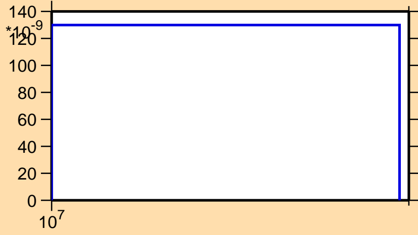
\sigma vs. E for ^{210}\text{Tl}(n,\text{nd})
