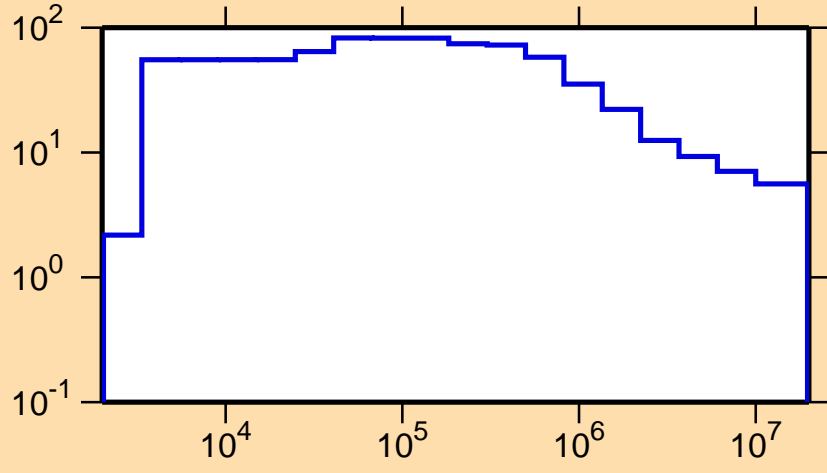
\Delta\sigma/\sigma vs. E for ^{210}\text{Tl}(n,\text{nonel.})
