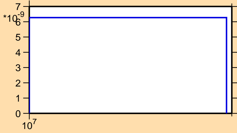
\sigma vs. E for ^{210}\text{Tl}(n,2np)
