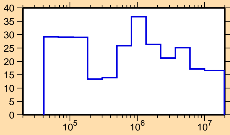
\Delta\sigma/\sigma vs. E for ^{210}\text{Tl}(n,\text{el.})
