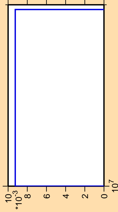
\Delta\sigma/\sigma vs. E for ^{210}\text{Tl} (mt 42)
