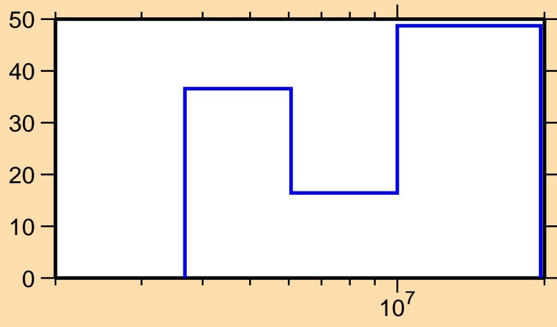
\Delta\sigma/\sigma vs. E for ^{210}\text{Tl}(n,2n)
