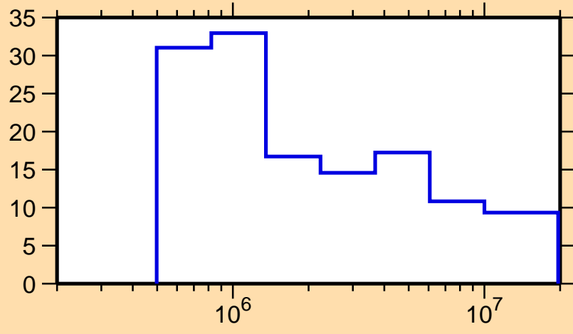
\Delta\sigma/\sigma vs. E for ^{210}\text{Tl}(n, \text{tot.})
