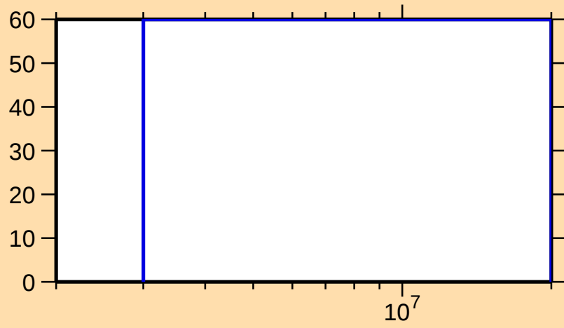
\Delta\sigma/\sigma vs. E for ^{243}\text{U}(\text{n},\gamma)
