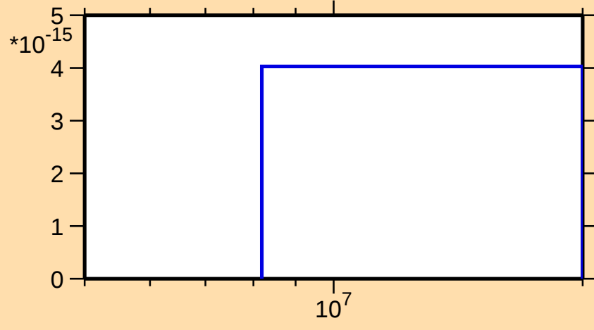
\sigma vs. E for ^{243}\text{U}(\text{mt 11})
