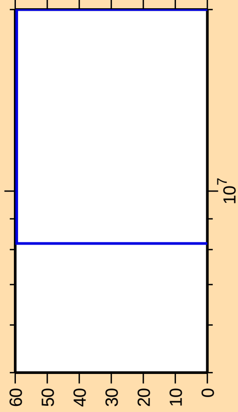
\Delta\sigma/\sigma vs. E for ^{243}\text{U}(\text{n,d})
