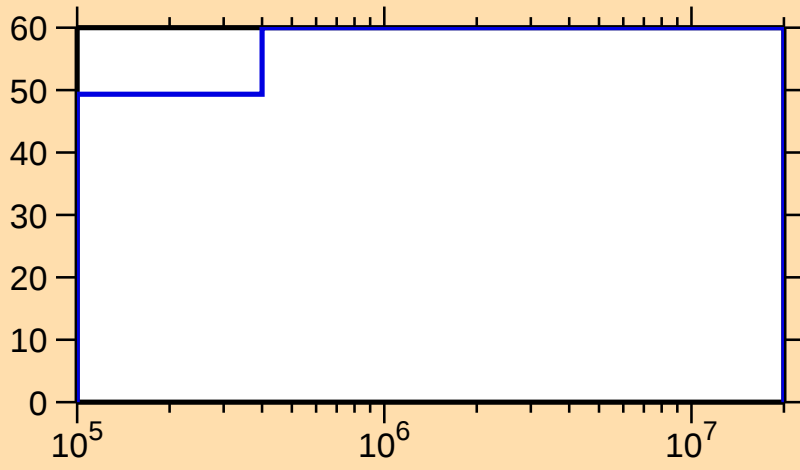
\Delta\sigma/\sigma vs. E for ^{243}\text{U}(\text{n},\text{f})
