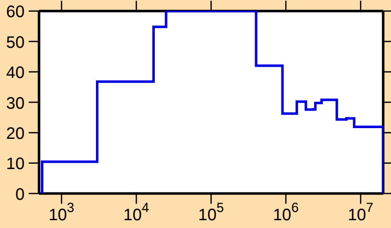
\Delta\sigma/\sigma vs. E for ^{243}\text{U}(\text{n},\text{nonel.})
