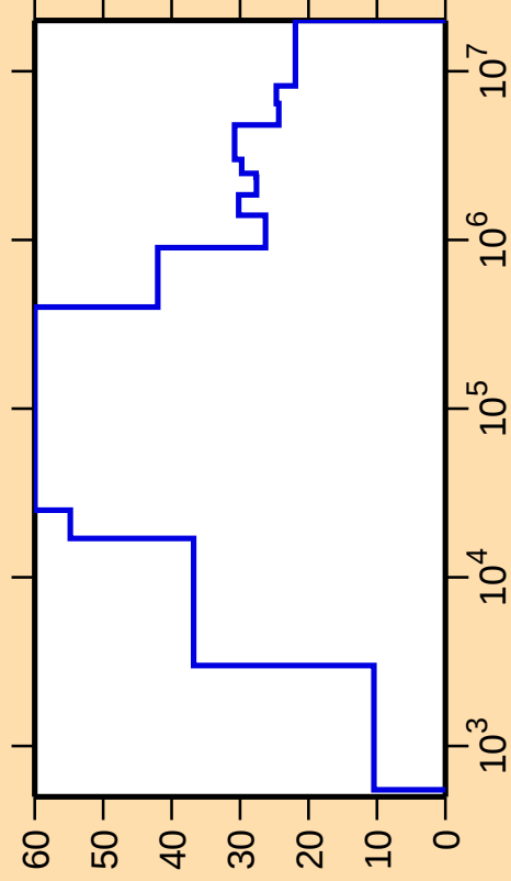
\Delta\sigma/\sigma vs. E for ^{243}\text{U}(\text{n,nonel.})
