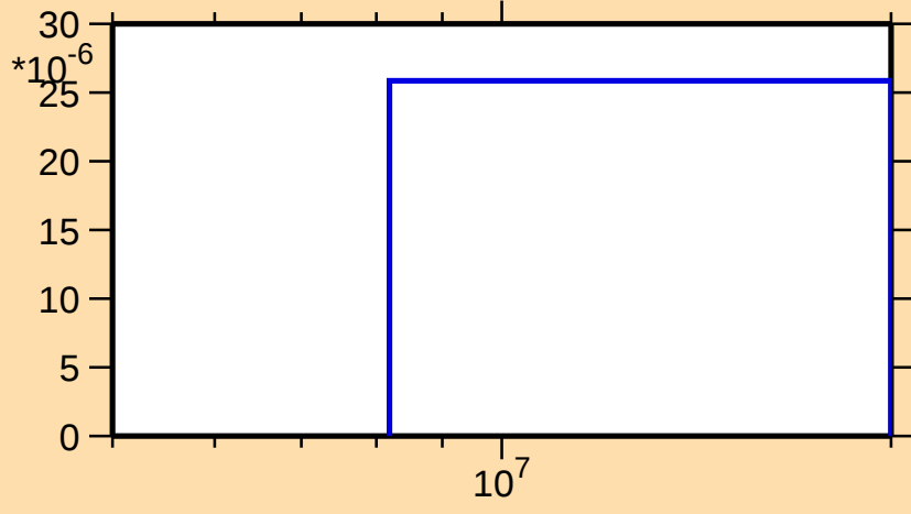
\sigma vs. E for ^{243}\text{U}(\text{n,t})
