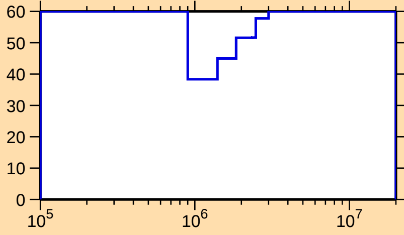
\Delta\sigma/\sigma vs. E for ^{243}\text{U}(\text{n},\text{inel.})
