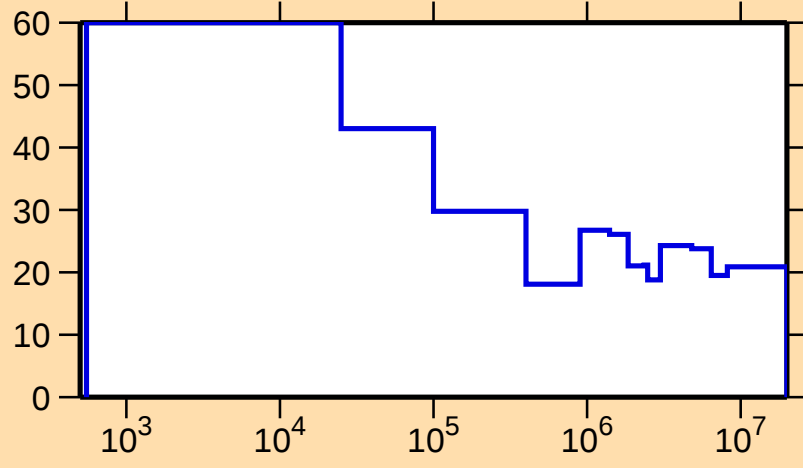
\Delta\sigma/\sigma vs. E for ^{243}\text{U}(\text{n,tot.})
