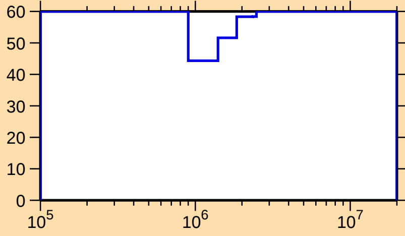
\Delta\sigma/\sigma vs. E for ^{243}\text{U}(n,n\text{cont.})
