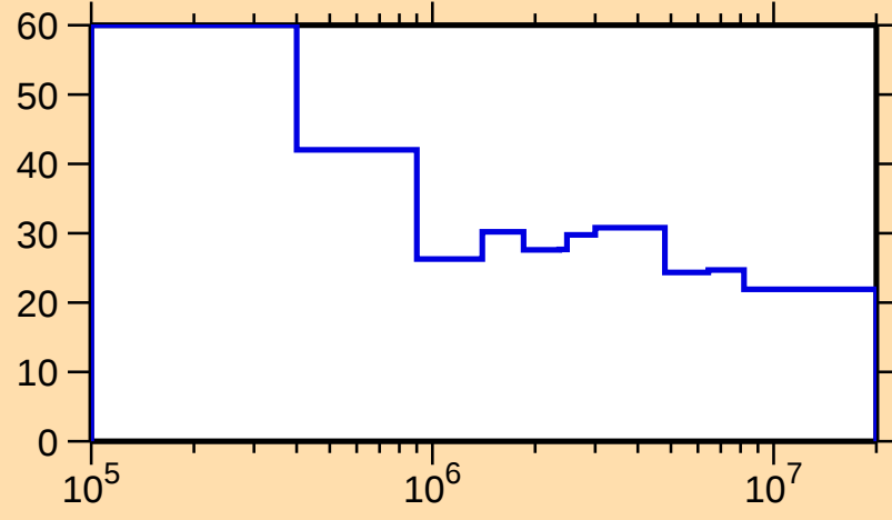
\Delta\sigma/\sigma vs. E for ^{243}\text{U}(\text{n,nonel.})
