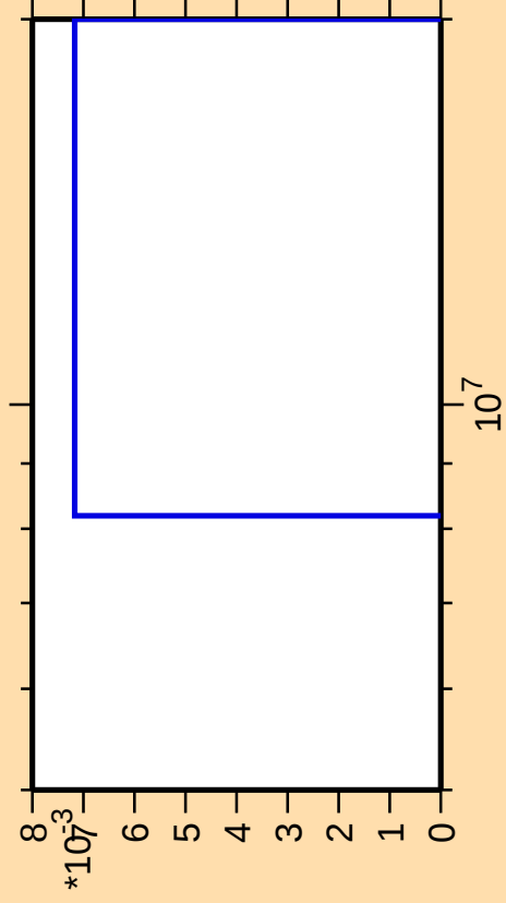
\Delta\sigma/\sigma vs. E for ^{243}\text{U}(\text{mt 11})
