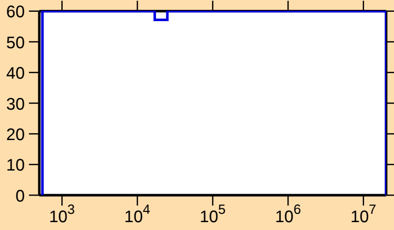
\Delta\sigma/\sigma vs. E for ^{243}\text{U}(n,\gamma)
