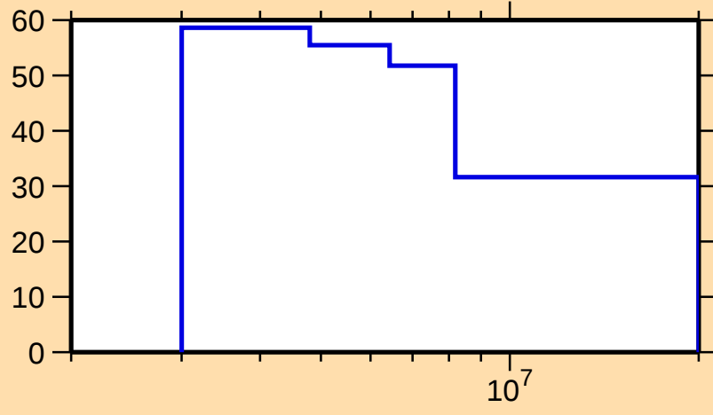
\Delta\sigma/\sigma vs. E for ^{243}\text{U}(n,2n)
