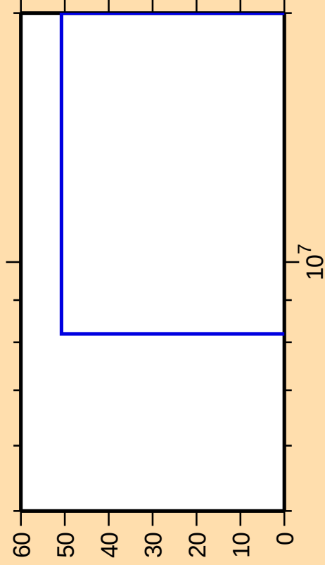
\Delta\sigma/\sigma vs. E for ^{243}\text{U}(\text{n},\text{nt})
