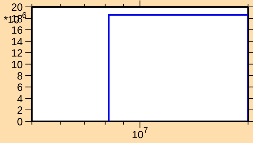
\sigma vs. E for ^{243}\text{U}(\text{n,d})
