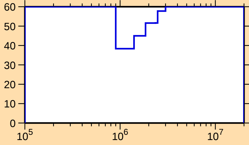
\Delta\sigma/\sigma vs. E for ^{243}\text{U}(\text{n},\text{inel.})
