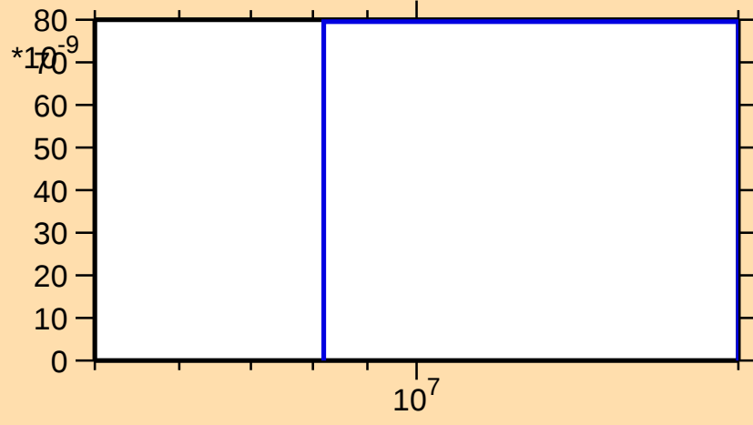
\sigma vs. E for ^{243}\text{U}(\text{n},\text{nt})
