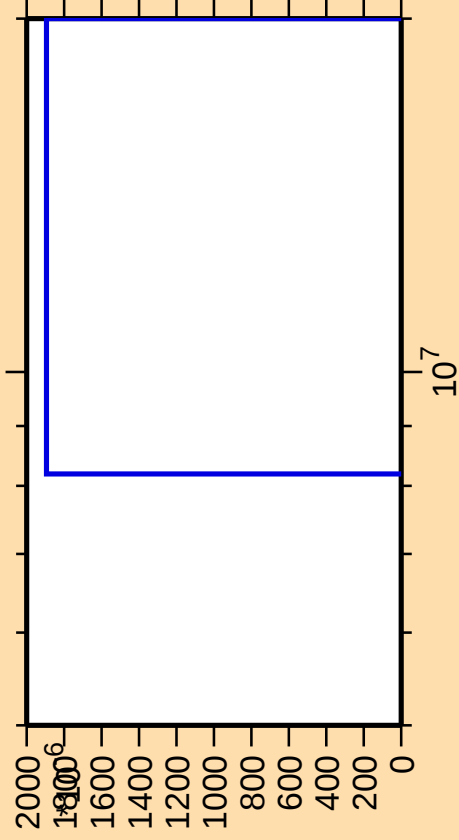
\Delta\sigma/\sigma vs. E for ^{243}\text{U}(n,\text{He3})
