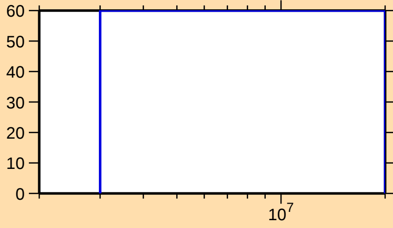
\Delta\sigma/\sigma vs. E for ^{243}\text{U}(\text{n,ncont.})
