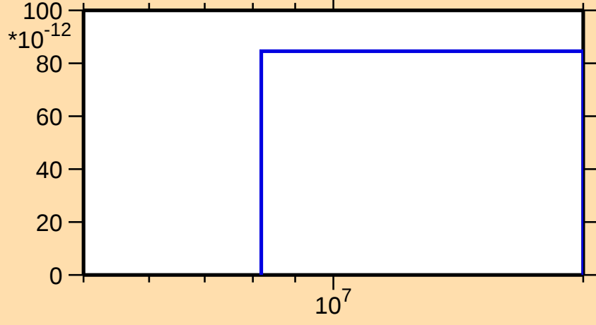
\sigma vs. E for ^{95}\text{Y}(n,2np)
