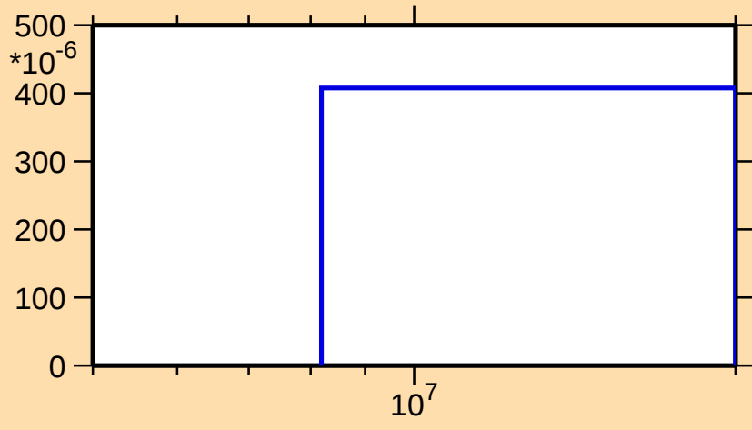
\sigma vs. E for ^{95}\text{Y}(n,d)
