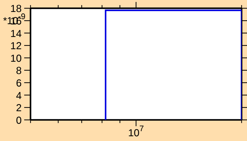
\sigma vs. E for ^{95}\text{Y}(\text{n},\text{nd})
