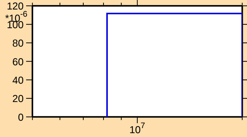
\sigma vs. E for ^{95}\text{Y}(n,np)
