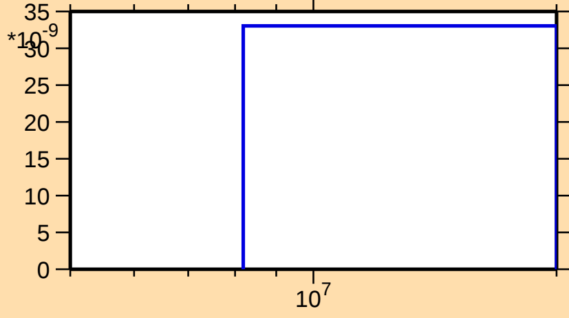
\sigma vs. E for ^{95}\text{Y}(n,nt)
