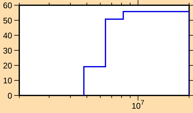
\Delta\sigma/\sigma vs. E for ^{95}\text{Y}(n,n\text{cont.})
