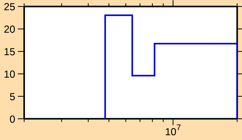
\Delta\sigma/\sigma vs. E for ^{95}\text{Y}(\text{n,el.})
