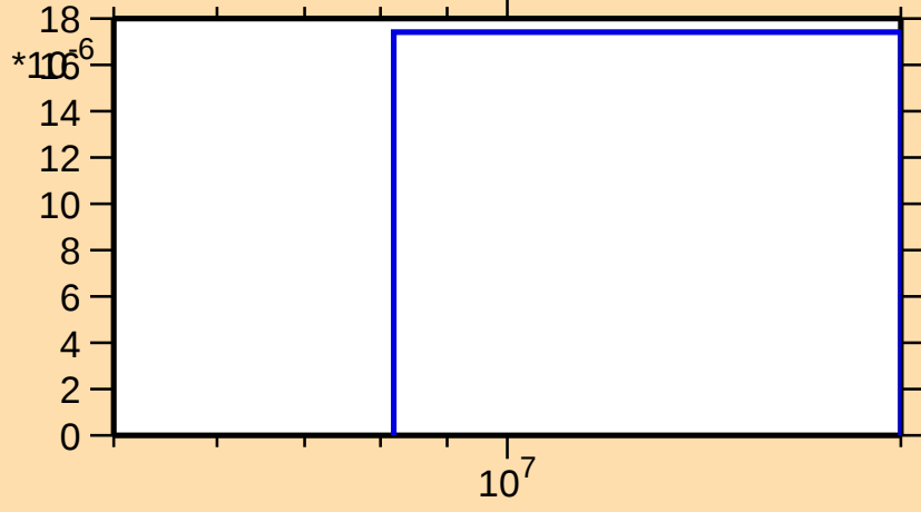
\sigma vs. E for ^{95}\text{Y}(n,n\alpha)
