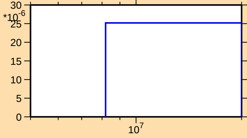
\sigma vs. E for ^{95}\text{Y}(n,t)
