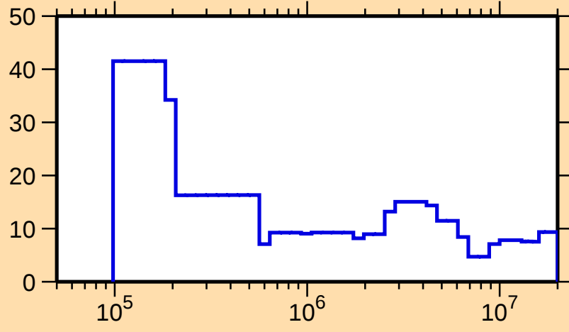
\Delta\sigma/\sigma vs. E for ^{175}\text{Yb}(n,\text{el.})
