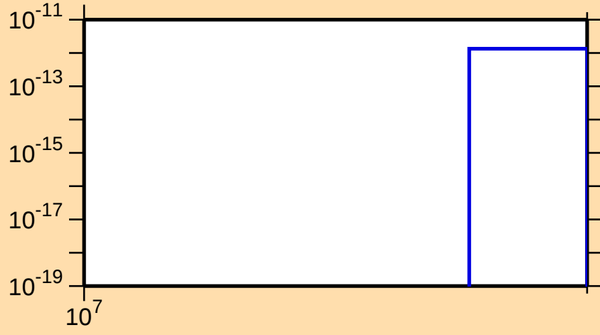
\sigma vs. E for ^{175}\text{Yb}(n,3n\alpha)
