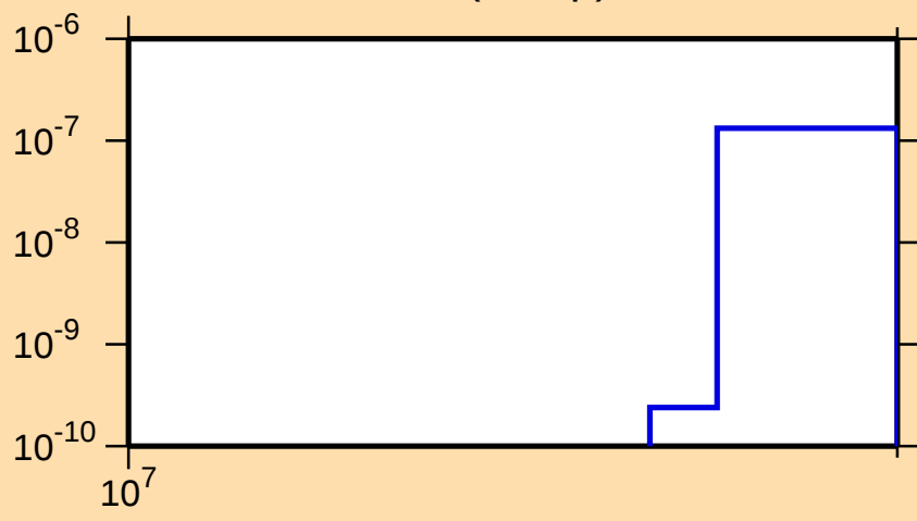
\sigma vs. E for ^{175}\text{Yb}(n,2np)
