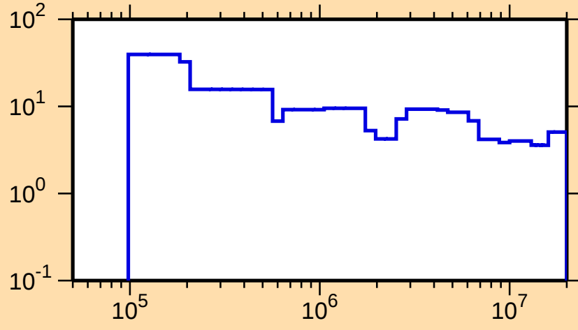
\Delta\sigma/\sigma vs. E for ^{175}\text{Yb}(n,\text{tot.})
