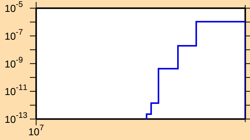
\sigma vs. E for ^{175}\text{Yb}(n,\text{nd})
