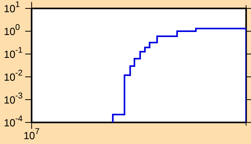
\sigma vs. E for ^{175}\text{Yb}(n,3n)
