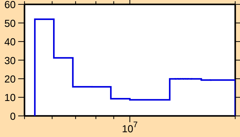
\Delta\sigma/\sigma vs. E for ^{175}\text{Yb}(n,2n)
