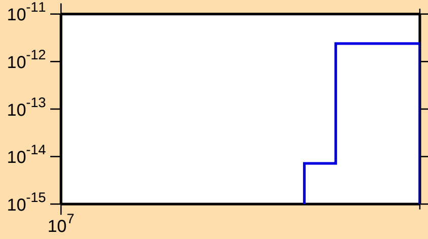
\sigma vs. E for ^{175}\text{Yb}(n,\text{He}3)
