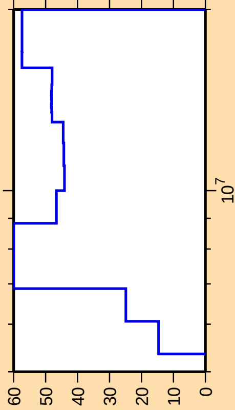
\Delta\sigma/\sigma vs. E for ^{175}\text{Yb}(n,n\text{cont.})
