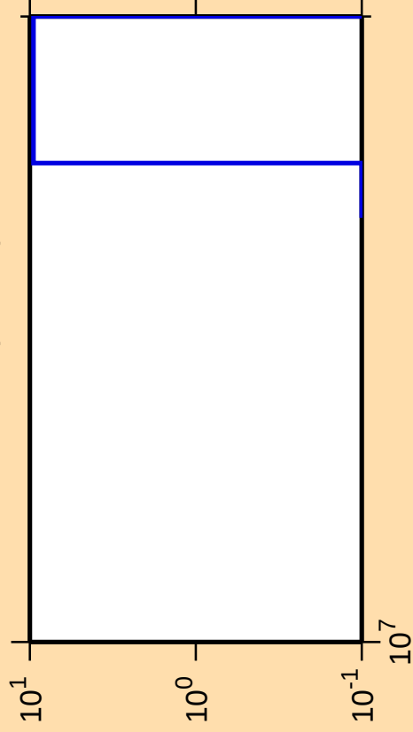
\Delta\sigma/\sigma vs. E for ^{175}\text{Yb}(n,3n\alpha)
