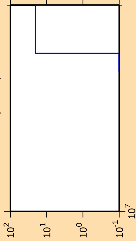
\Delta\sigma/\sigma vs. E for ^{175}\text{Yb}(n,\text{He}3)
