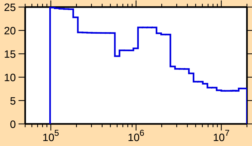
\Delta\sigma/\sigma vs. E for ^{175}\text{Yb}(n,\text{nonel.})
