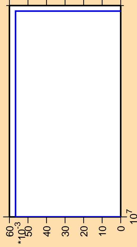
\Delta\sigma/\sigma vs. E for ^{175}\text{Yb}(n,3n\alpha)
