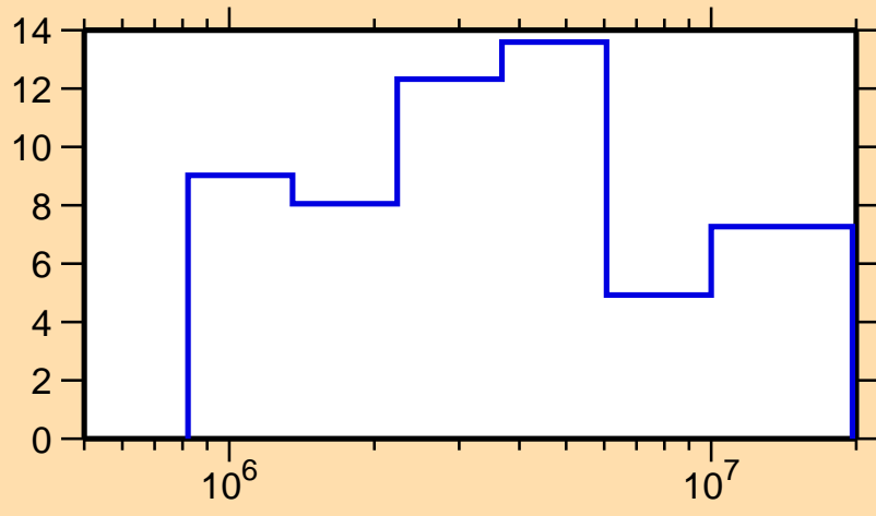
\Delta\sigma/\sigma vs. E for ^{175}\text{Yb}(n, el.)
