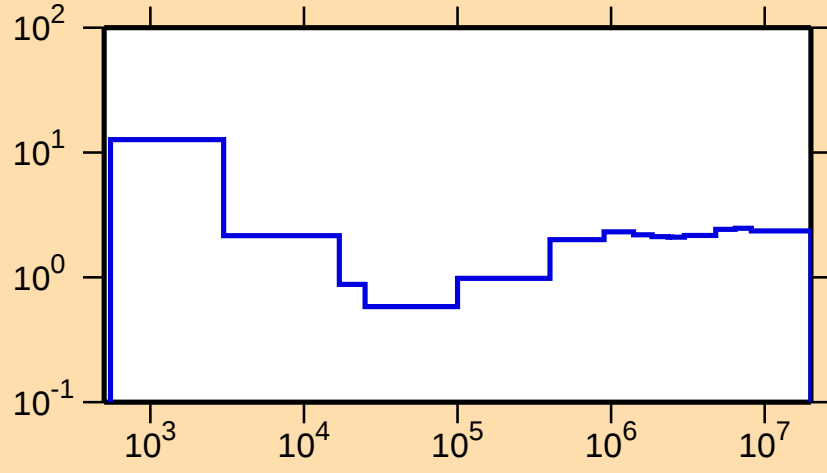
\sigma vs. E for ^{175}\text{Yb}(n,\text{nonel.})
