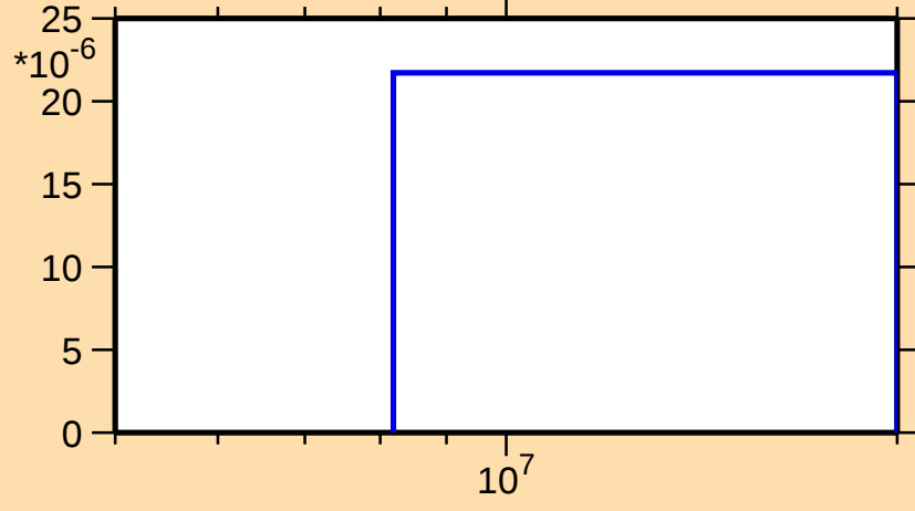
\sigma vs. E for ^{175}\text{Yb}(n,t)
