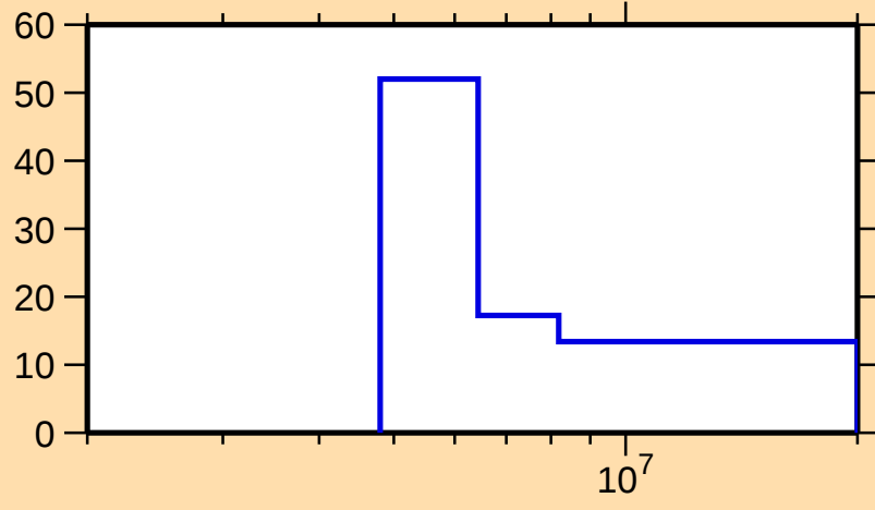
\Delta\sigma/\sigma vs. E for ^{175}\text{Yb}(n,2n)
