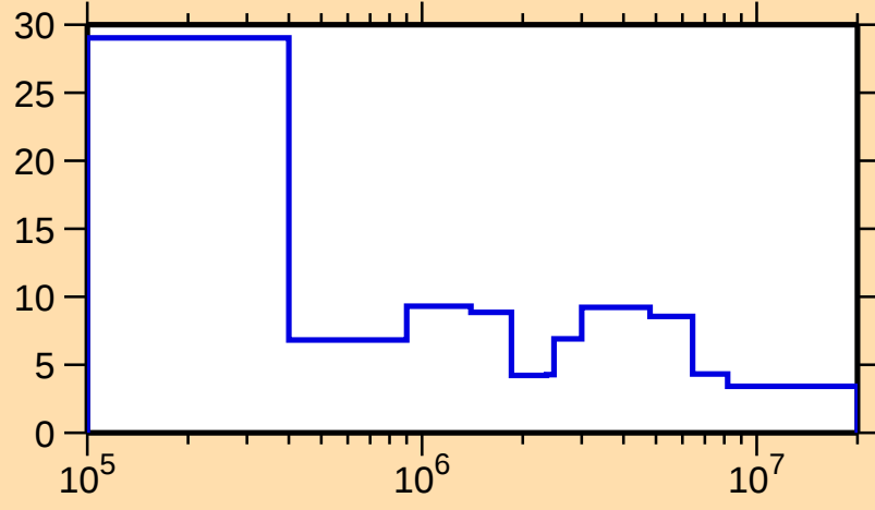
\Delta\sigma/\sigma vs. E for ^{175}\text{Yb}(n,\text{tot.})
