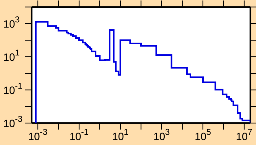
\sigma vs. E for ^{175}\text{Yb}(n,\gamma)
