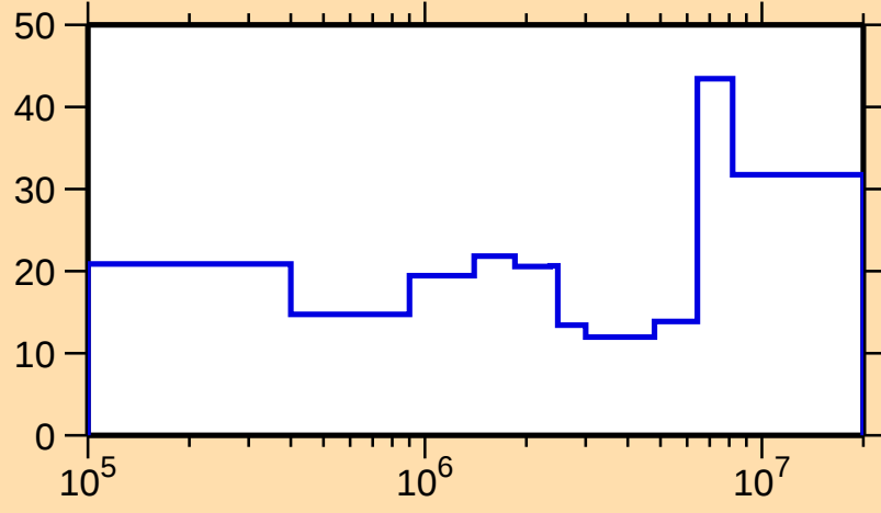
\Delta\sigma/\sigma vs. E for ^{175}\text{Yb}(n,\text{inel.})
