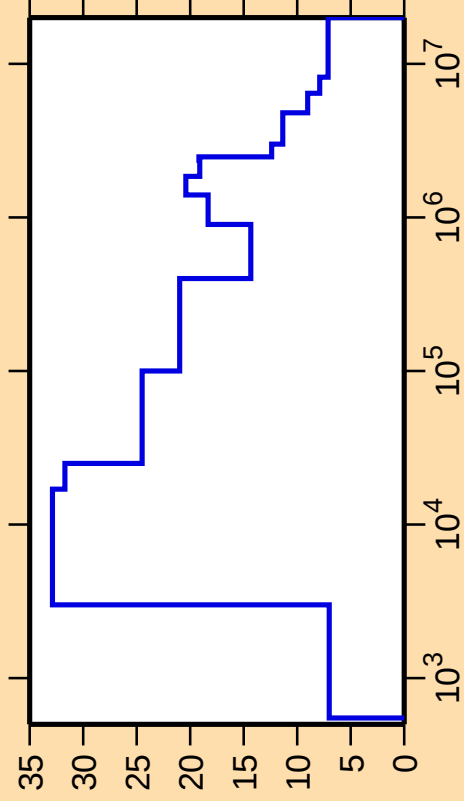
\Delta\sigma/\sigma vs. E for ^{175}\text{Yb}(n,\text{nonel.})
