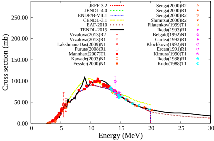
^{27}\text{Al}(n,p)^{27}\text{Mg}
