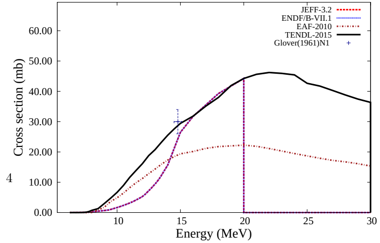
^{27}\text{Al}(n,d)^{26}\text{Mg}
