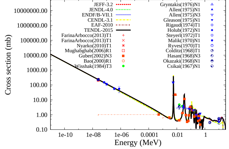
^{27}\text{Al}(n,g)^{28}\text{Al}
