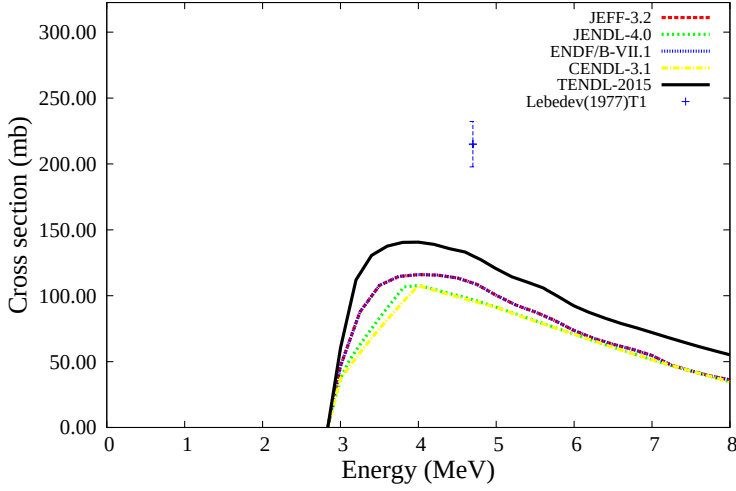
^{27}\text{Al}(n,g)^{28}\text{Al}
