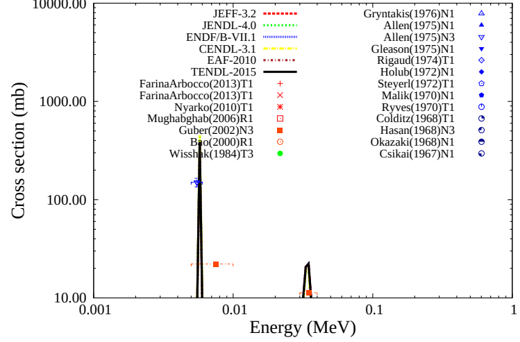
^{27}\text{Al}(n,d)^{26}\text{Mg}
