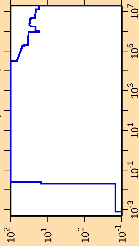
\Delta\sigma/\sigma vs. E for ^{214}\text{Ac}(n,\text{nonel.})
