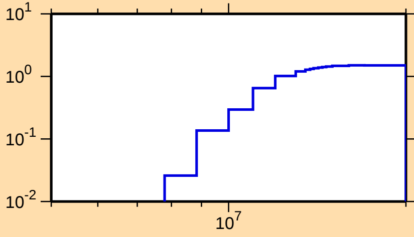
\sigma vs. E for ^{214}\text{Ac}(n,2n)
