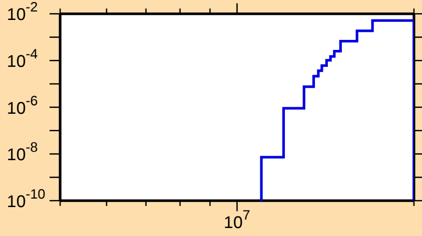
\sigma vs. E for ^{214}\text{Ac}(n,2np)
