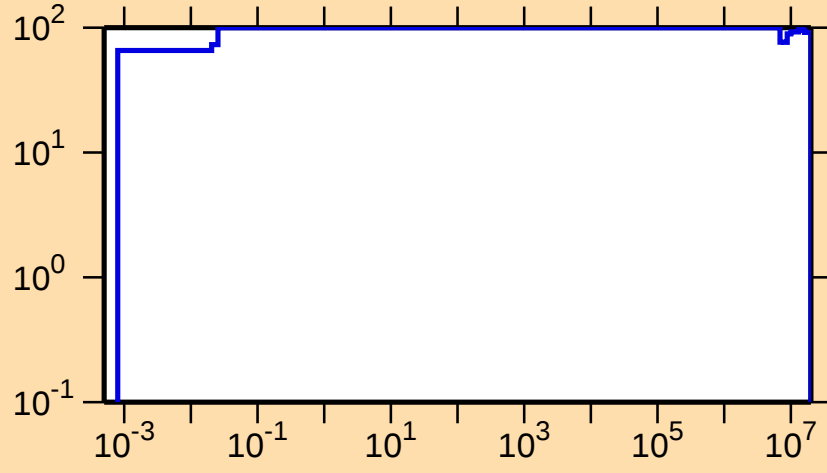
\Delta\sigma/\sigma vs. E for ^{214}\text{Ac}(n,p)
