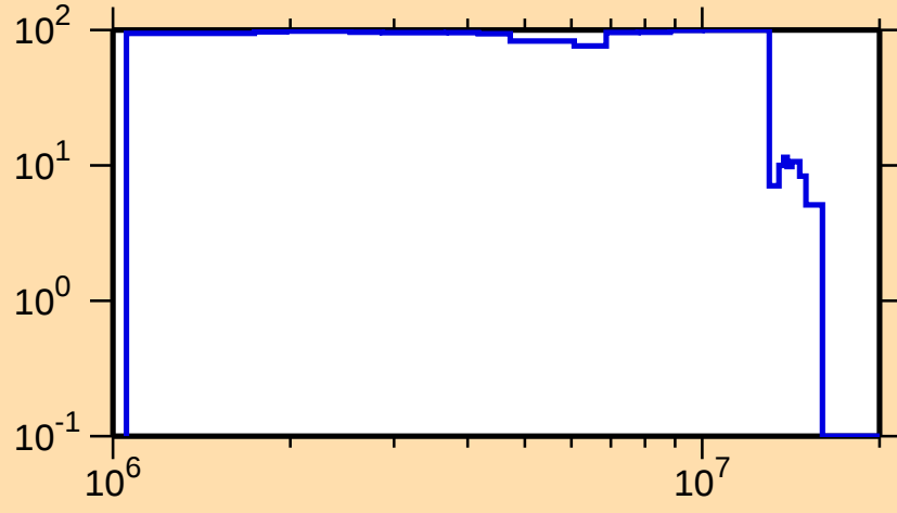
\Delta\sigma/\sigma vs. E for ^{214}\text{Ac}(n,n_1)
