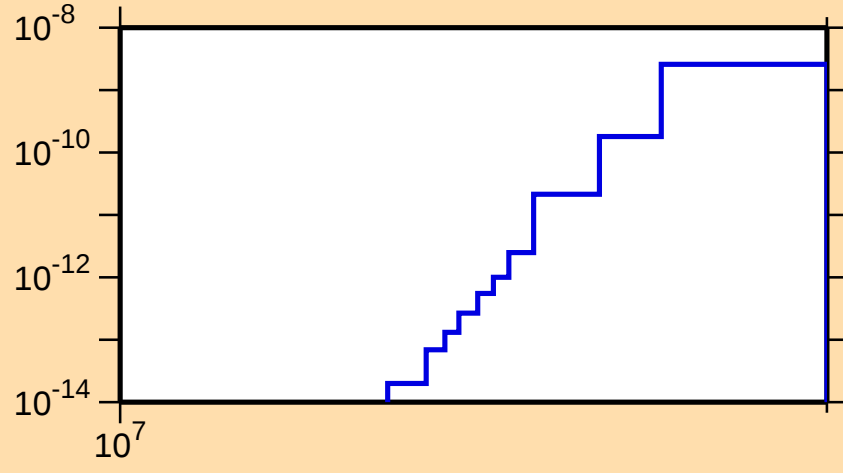
\sigma vs. E for ^{214}\text{Ac}(\text{mt } 34)
