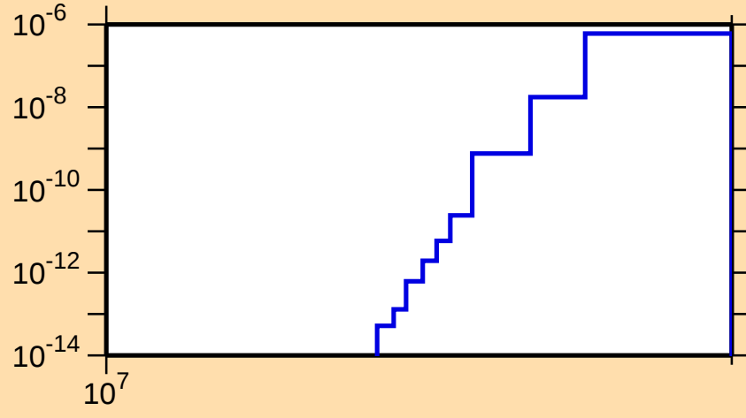
\sigma vs. E for ^{214}\text{Ac}(n,nt)
