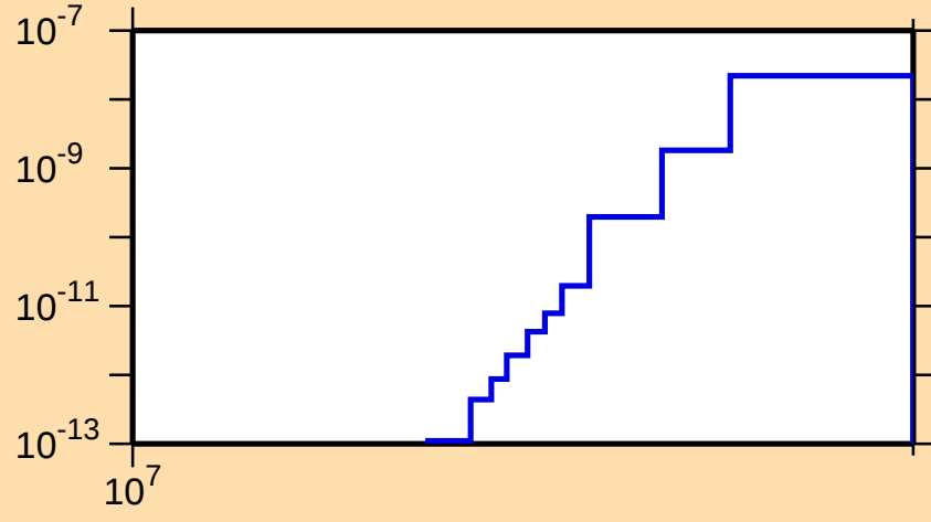
\sigma vs. E for ^{214}\text{Ac}(n,\text{pt})
