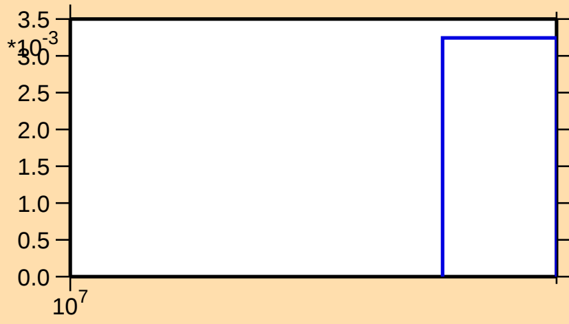
\sigma vs. E for ^{214}\text{Ac}(n,3n)
