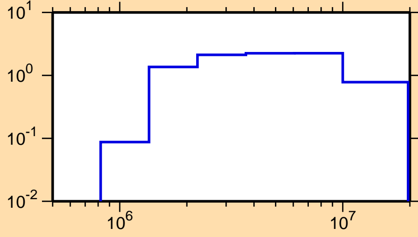
\sigma vs. E for ^{214}\text{Ac}(n,n\text{cont.})
