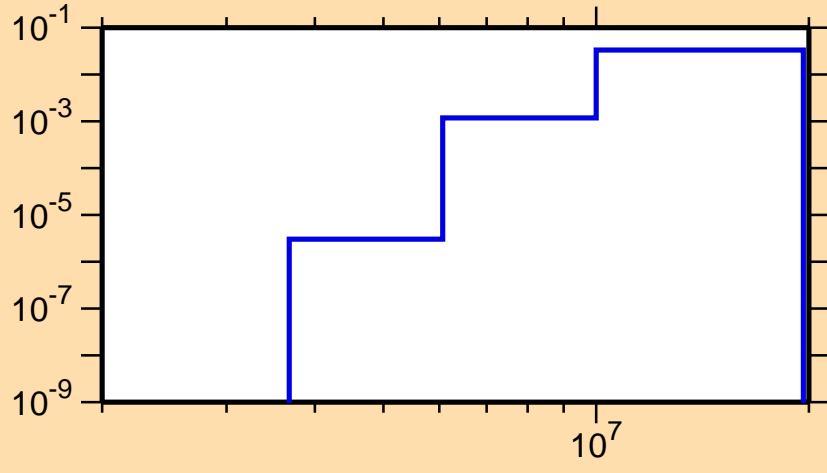
\sigma vs. E for ^{214}\text{Ac}(n,np)
