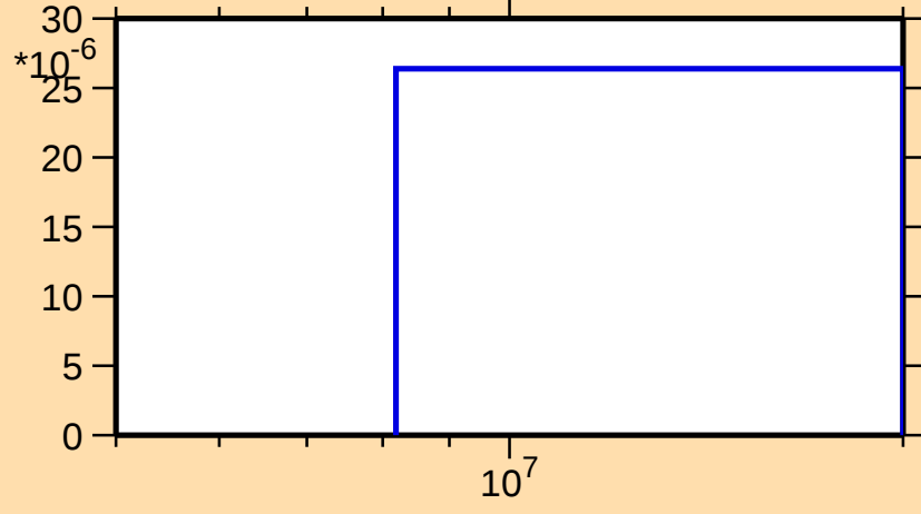
\sigma vs. E for ^{214}\text{Ac}(n,3n)
