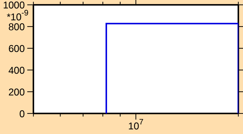
\sigma vs. E for ^{214}\text{Ac}(n,\text{nd})
