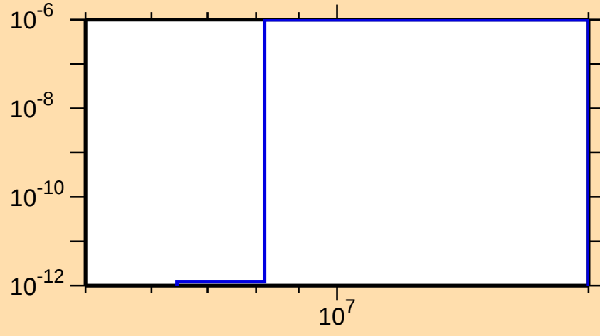
\sigma vs. E for ^{214}\text{Ac}(n,\text{He3})
