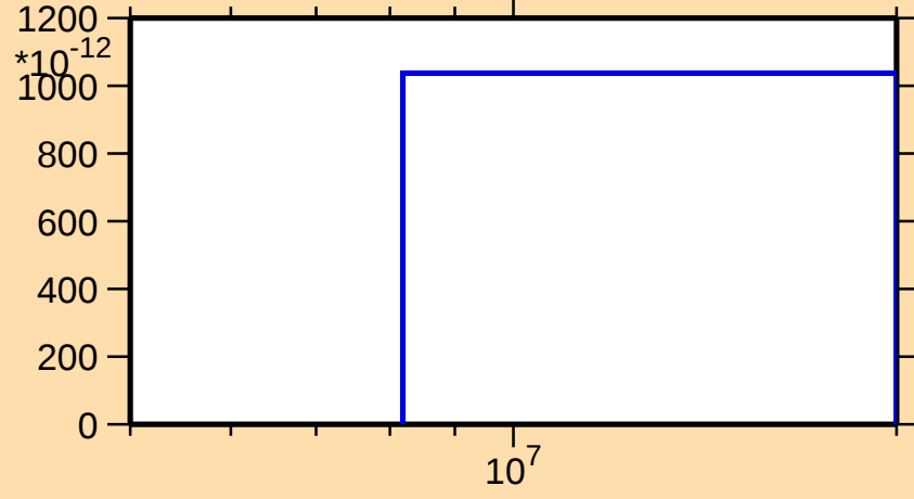
\sigma vs. E for ^{214}\text{Ac}(n,\text{pd})
