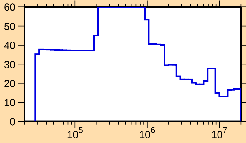
\Delta\sigma/\sigma vs. E for ^{225}\text{Ac}(n,\text{el.})
