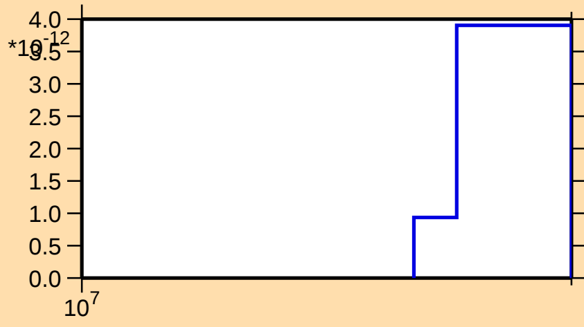
\sigma vs. E for ^{225}\text{Ac}(\text{mt117})
