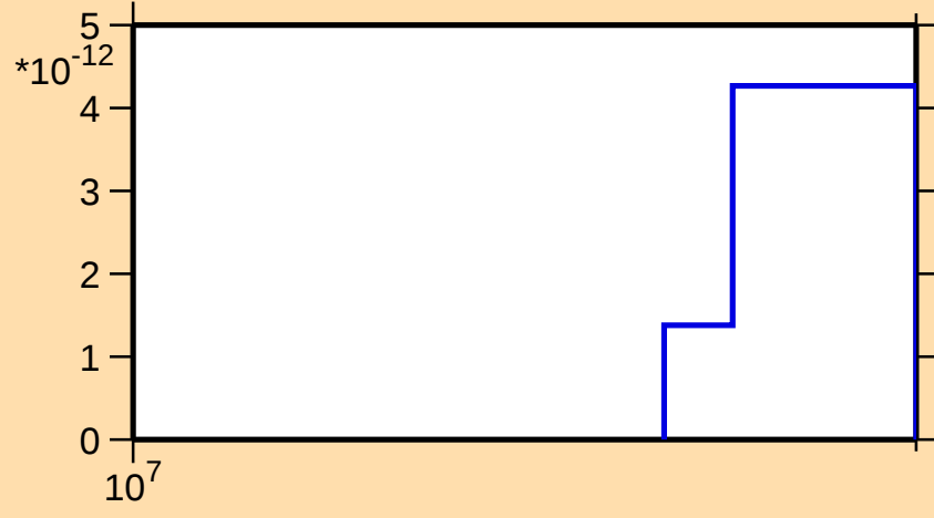
\sigma vs. E for ^{225}\text{Ac}(n,p\alpha)
