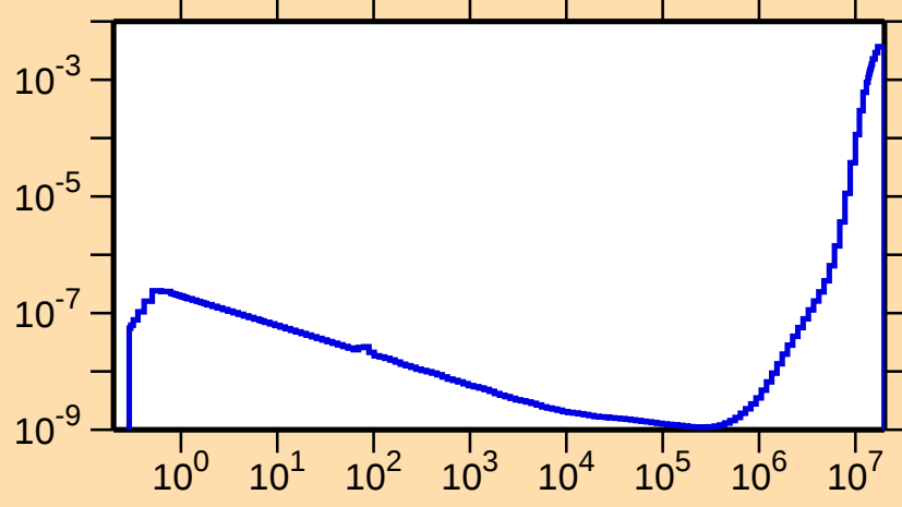
\sigma vs. E for ^{225}\text{Ac}(n,\alpha)
