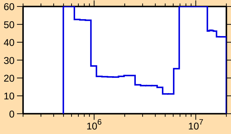
\Delta\sigma/\sigma vs. E for ^{227}\text{Ac}(n,\text{inel.})
