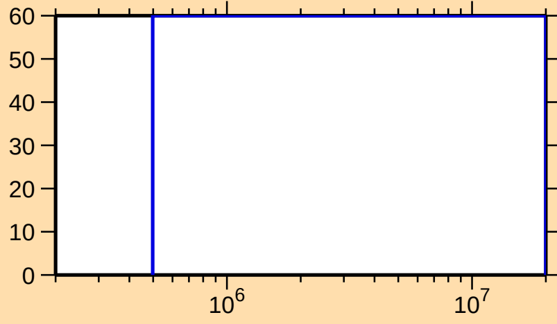
\Delta\sigma/\sigma vs. E for ^{227}\text{Ac}(n,\text{f})
