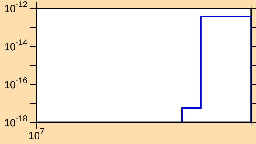
\sigma vs. E for ^{227}\text{Ac}(\text{mt } 42)
