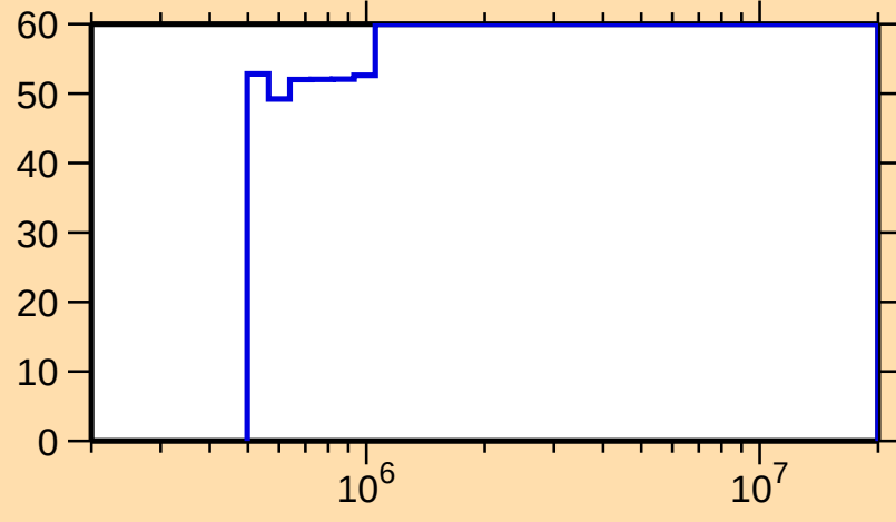
\Delta\sigma/\sigma vs. E for ^{227}\text{Ac}(n,n_1)
