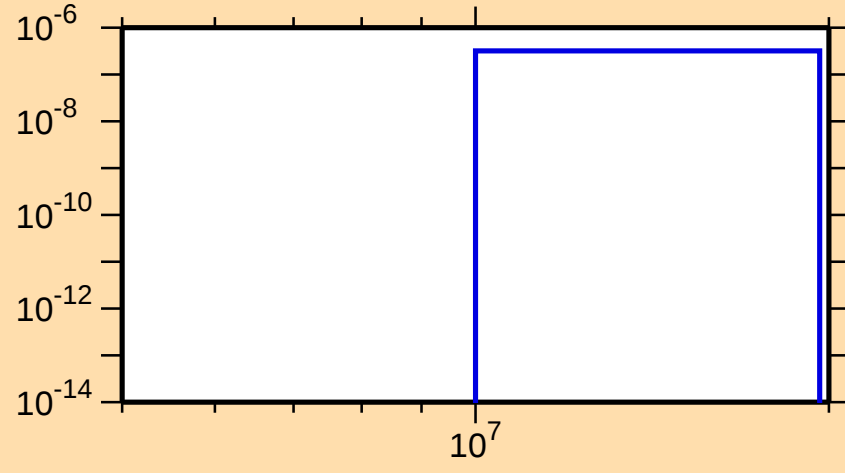
\sigma vs. E for ^{227}\text{Ac}(n,\text{nt})
