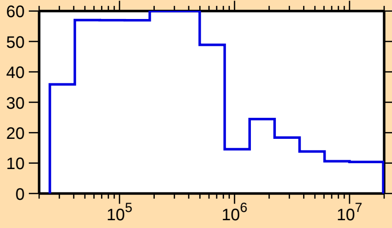
\Delta\sigma/\sigma vs. E for ^{227}\text{Ac}(\text{n,nonel.})
