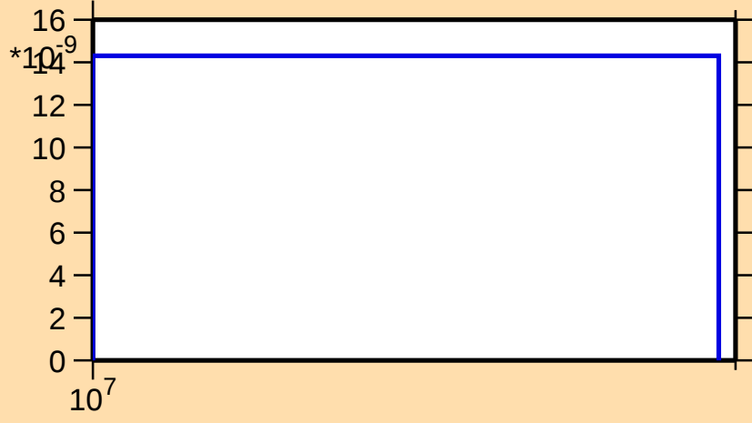
\sigma vs. E for ^{227}\text{Ac}(n,2np)
