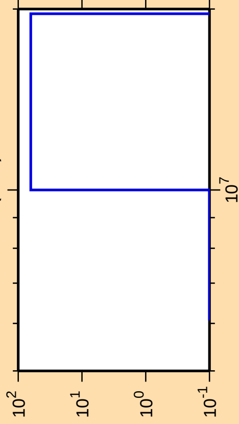
\Delta\sigma/\sigma vs. E for ^{227}\text{Ac}(n,\text{nt})
