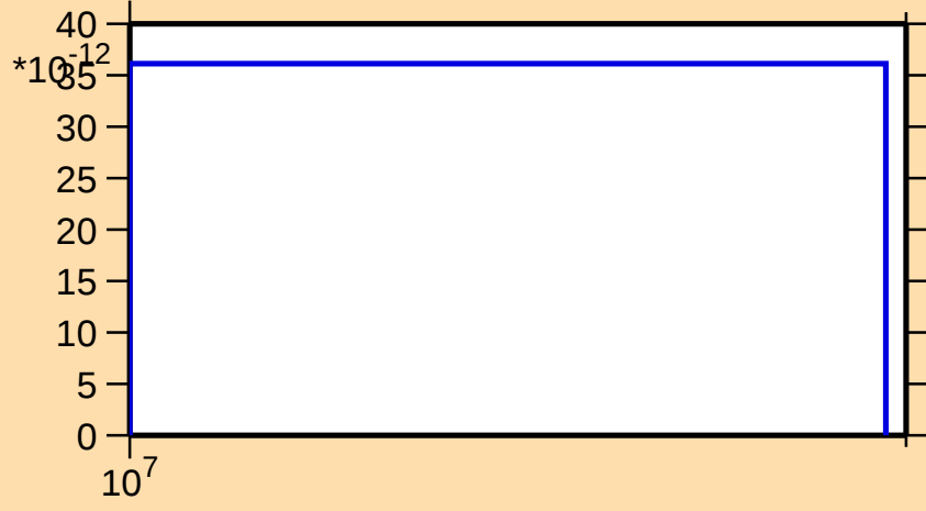
\sigma vs. E for ^{227}\text{Ac}(n,3n\alpha)
