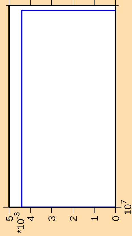
\Delta\sigma/\sigma vs. E for ^{227}\text{Ac}(\text{mt } 42)
