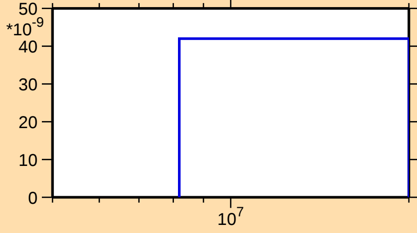
\sigma vs. E for ^{227}\text{Ac}(\text{n},\text{nd})
