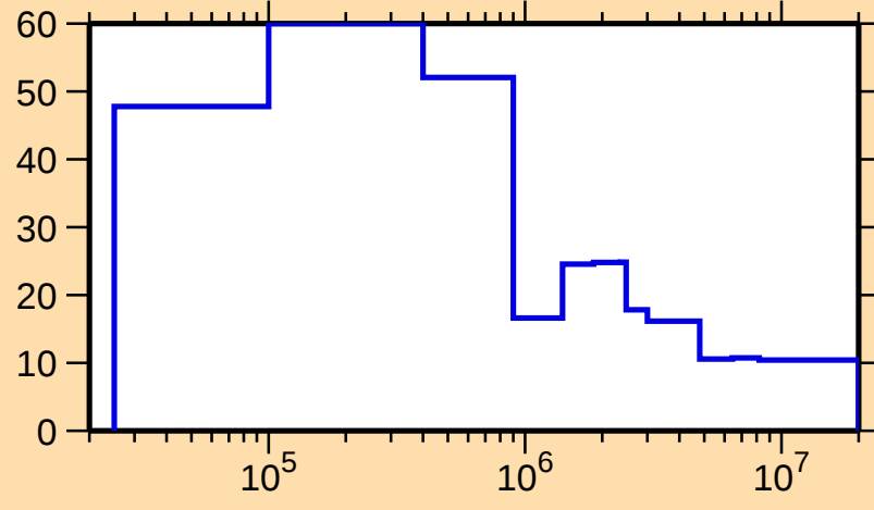
\Delta\sigma/\sigma vs. E for ^{227}\text{Ac}(n,\text{nonel.})
