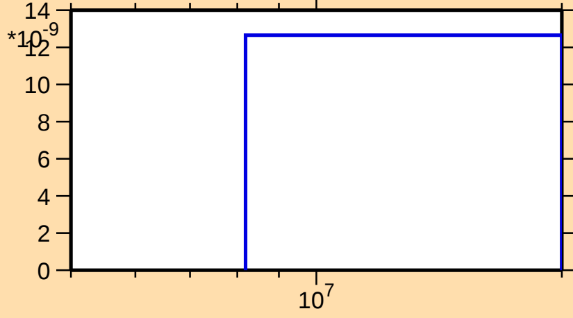
\sigma vs. E for ^{227}\text{Ac}(n,2np)
