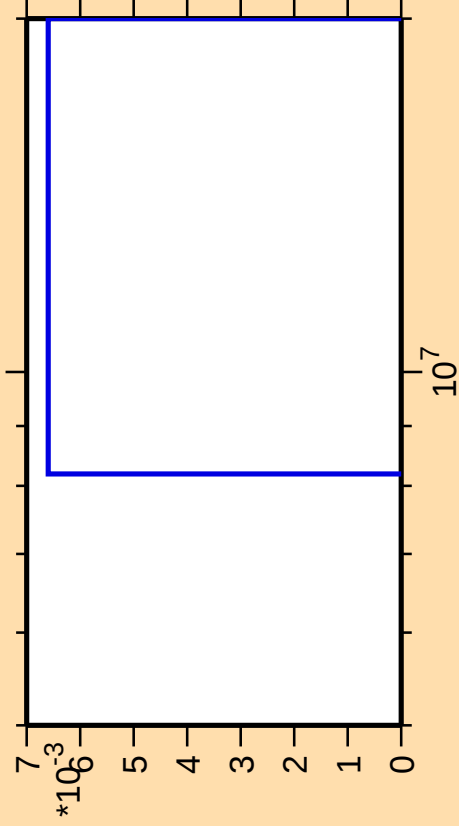
\Delta\sigma/\sigma vs. E for ^{227}\text{Ac}(\text{mt } 42)
