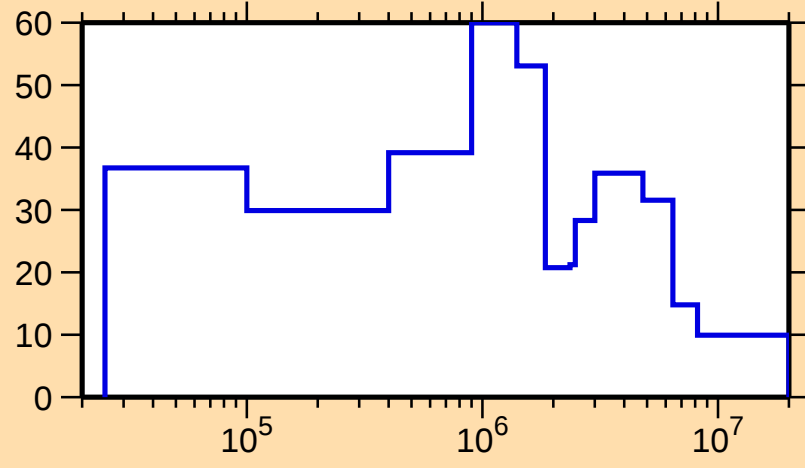
\Delta\sigma/\sigma vs. E for ^{227}\text{Ac}(\text{n,el.})
