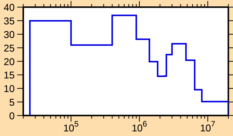
\Delta\sigma/\sigma vs. E for ^{227}\text{Ac}(n,\text{tot.})
