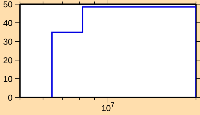
\Delta\sigma/\sigma vs. E for ^{227}\text{Ac}(n,2n)
