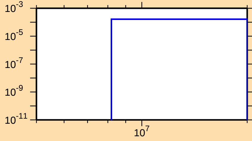
\sigma vs. E for ^{227}\text{Ac}(n,np)
