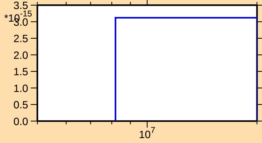
\sigma vs. E for ^{227}\text{Ac}(\text{mt } 42)
