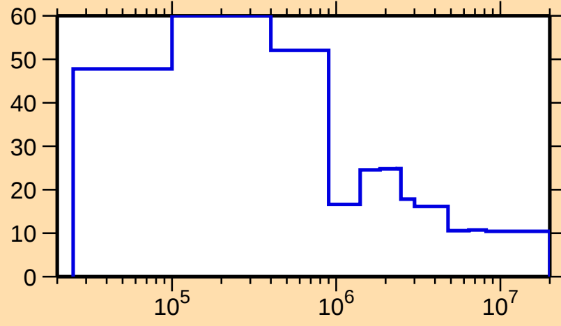
\Delta\sigma/\sigma vs. E for ^{227}\text{Ac}(n,\text{nonel.})
