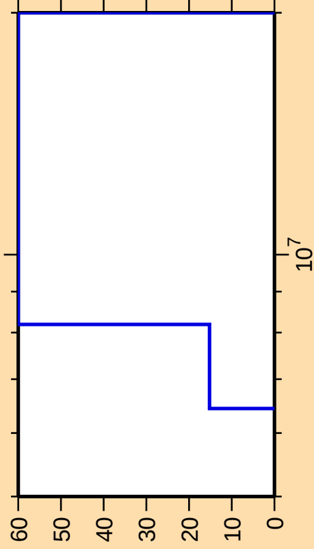
\Delta\sigma/\sigma vs. E for ^{227}\text{Ac}(n,d)
