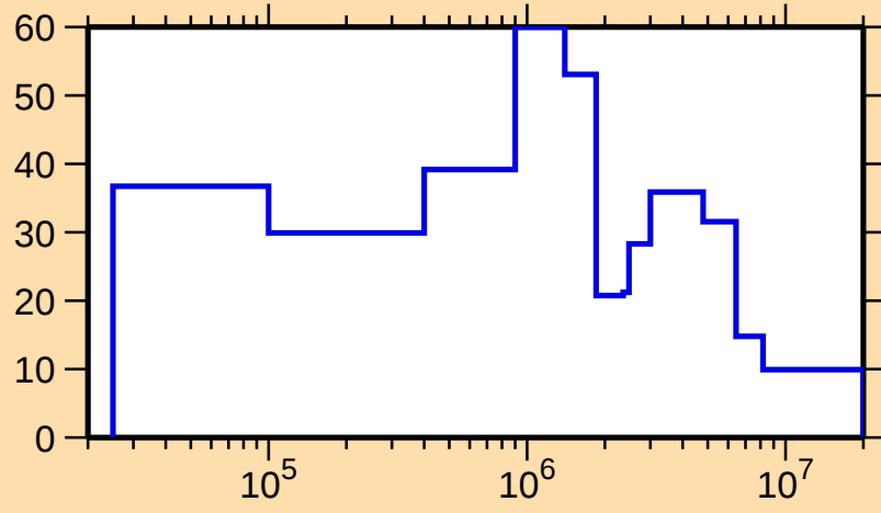
\Delta\sigma/\sigma vs. E for ^{227}\text{Ac}(n,\text{el.})
