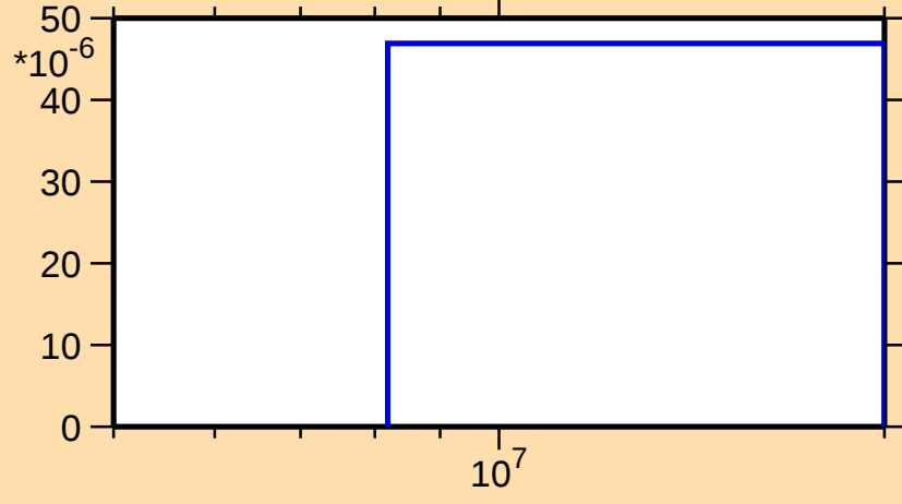
\sigma vs. E for ^{227}\text{Ac}(n,t)
