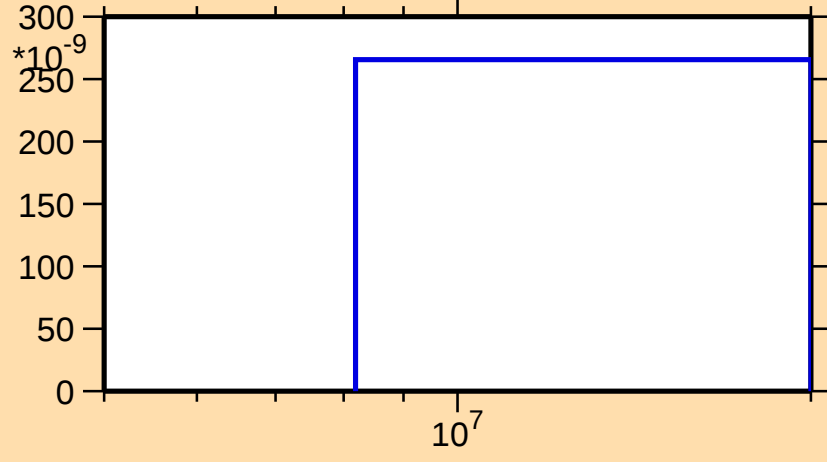
\sigma vs. E for ^{227}\text{Ac}(n,nt)
