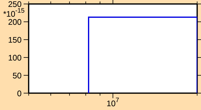
\sigma vs. E for ^{227}\text{Ac}(n,\text{He}3)
