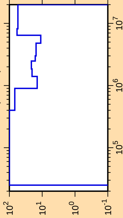
\Delta\sigma/\sigma vs. E for ^{227}\text{Ac}(\text{n,inel.})
