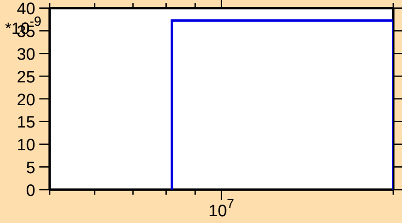
\sigma vs. E for ^{227}\text{Ac}(n,2n\alpha)
