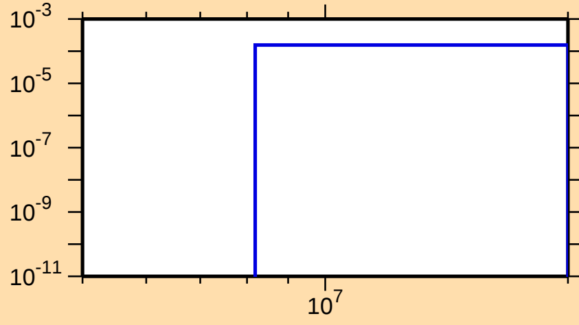
\sigma vs. E for ^{227}\text{Ac}(n,d)
