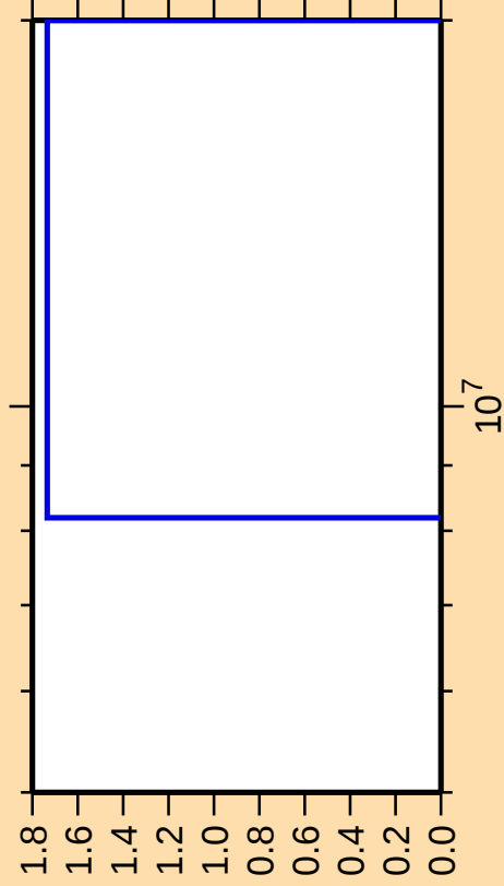
\Delta\sigma/\sigma vs. E for ^{227}\text{Ac}(n,\text{He}3)
