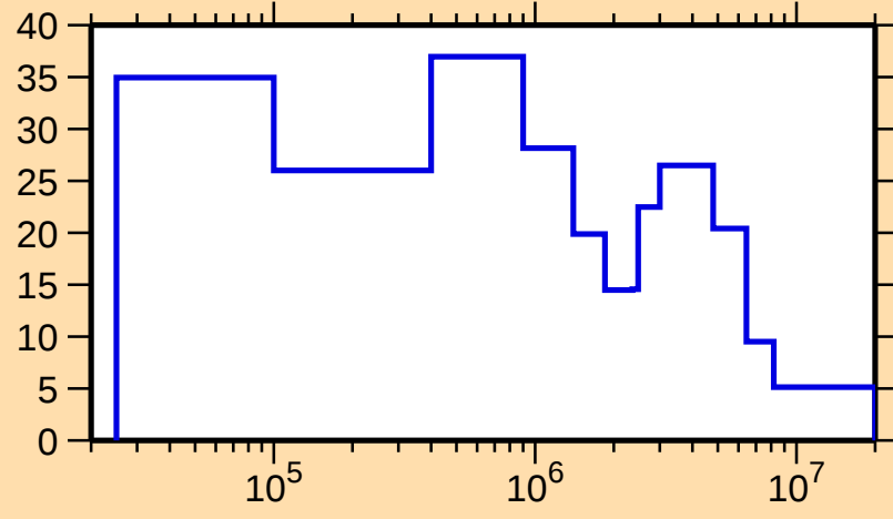
\Delta\sigma/\sigma vs. E for ^{227}\text{Ac}(\text{n,tot.})
