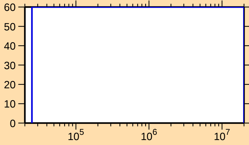
\Delta\sigma/\sigma vs. E for ^{227}\text{Ac}(n,f)
