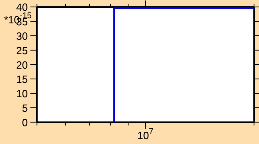
\sigma vs. E for ^{227}\text{Ac}(\text{mt } 11)
