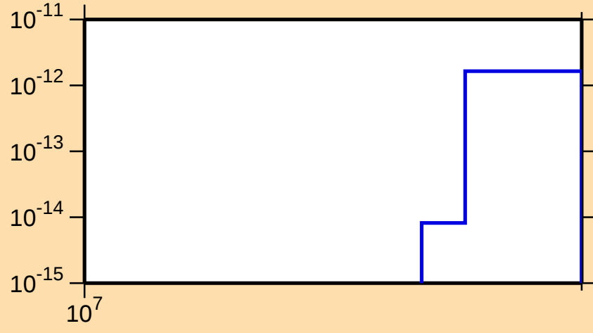
\sigma vs. E for ^{236}\text{Ac}(n,3n\alpha)
