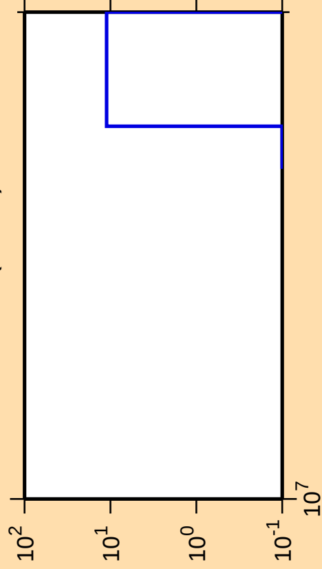
\Delta\sigma/\sigma vs. E for ^{236}\text{Ac}(\text{mt } 11)
