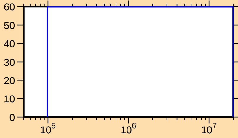
\Delta\sigma/\sigma vs. E for ^{236}\text{Ac}(n,n_1)
