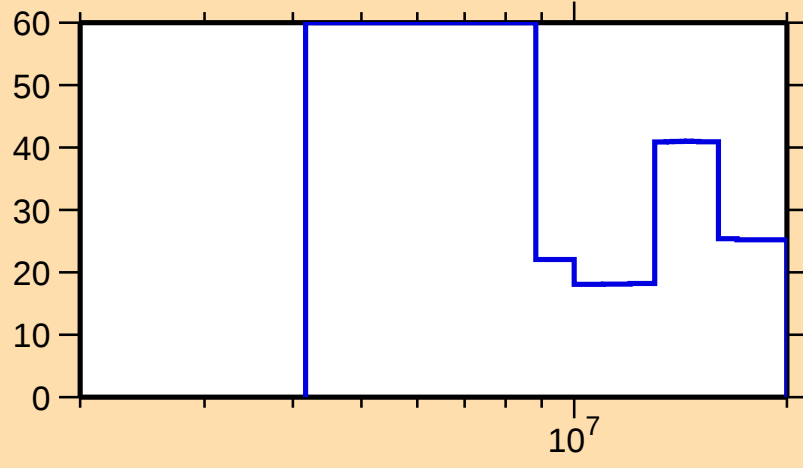
\Delta\sigma/\sigma vs. E for ^{236}\text{Ac}(n,2n)
