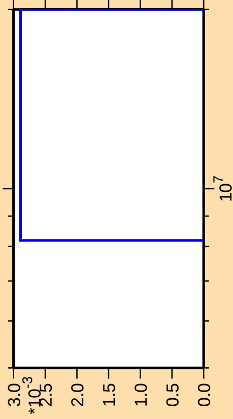
\Delta\sigma/\sigma vs. E for ^{236}\text{Ac}(\text{mt } 42)
