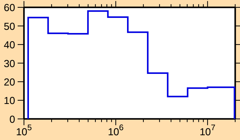
\Delta\sigma/\sigma vs. E for ^{237}\text{Ac}(n,\text{inel.})
