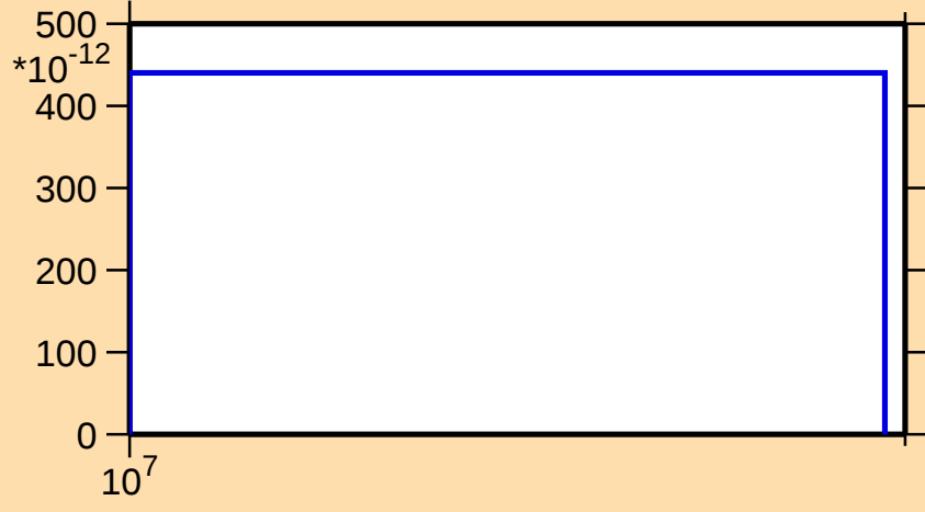
\sigma vs. E for ^{237}\text{Ac}(n,2n\alpha)
