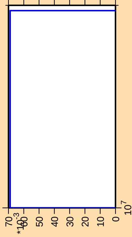
\Delta\sigma/\sigma vs. E for ^{237}\text{Ac}(\text{mt } 11)
