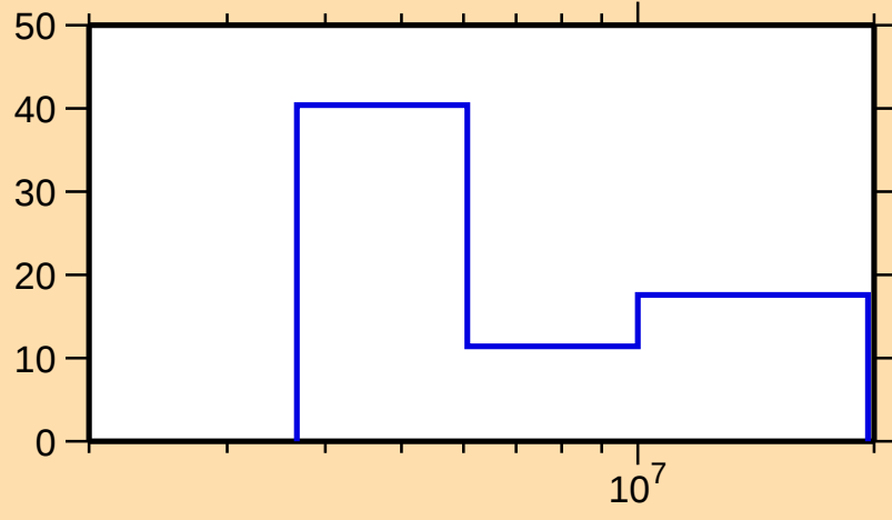
\Delta\sigma/\sigma vs. E for ^{237}\text{Ac}(n,\text{el.})
