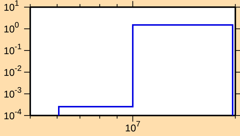
\sigma vs. E for ^{237}\text{Ac}(n,3n)
