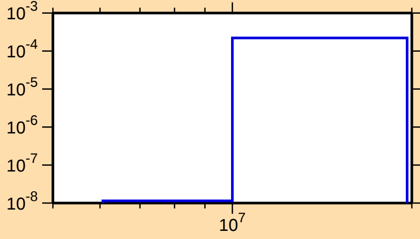
\sigma vs. E for ^{237}\text{Ac}(n,p)
