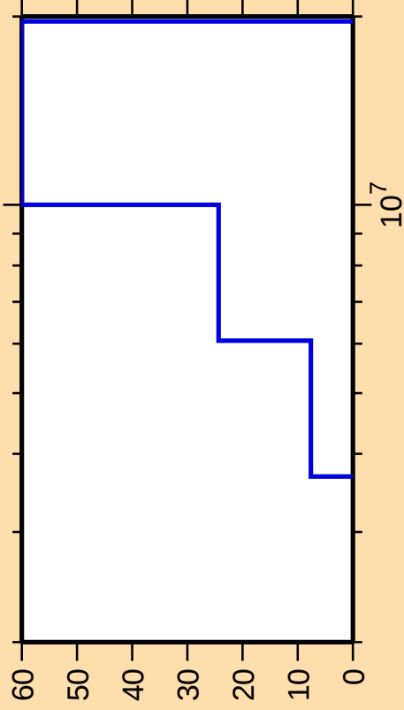
\Delta\sigma/\sigma vs. E for ^{237}\text{Ac}(n,n\text{cont.})
