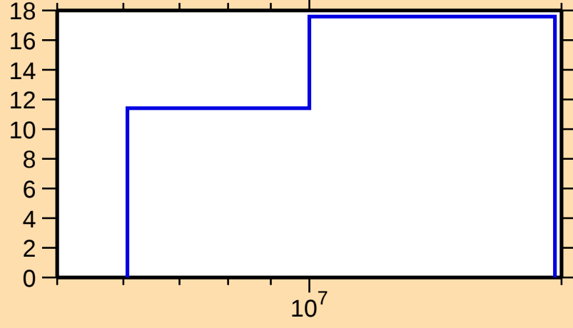
\Delta\sigma/\sigma vs. E for ^{237}\text{Ac}(n,\text{el.})
