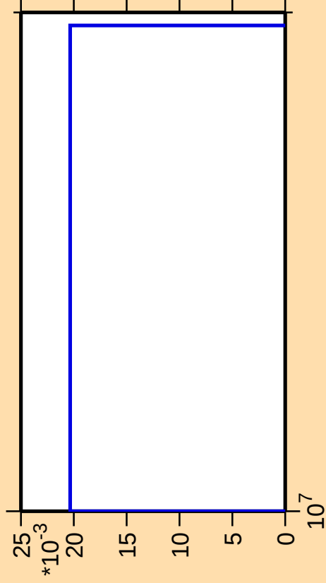
\Delta\sigma/\sigma vs. E for ^{237}\text{Ac}(n,3n\alpha)
