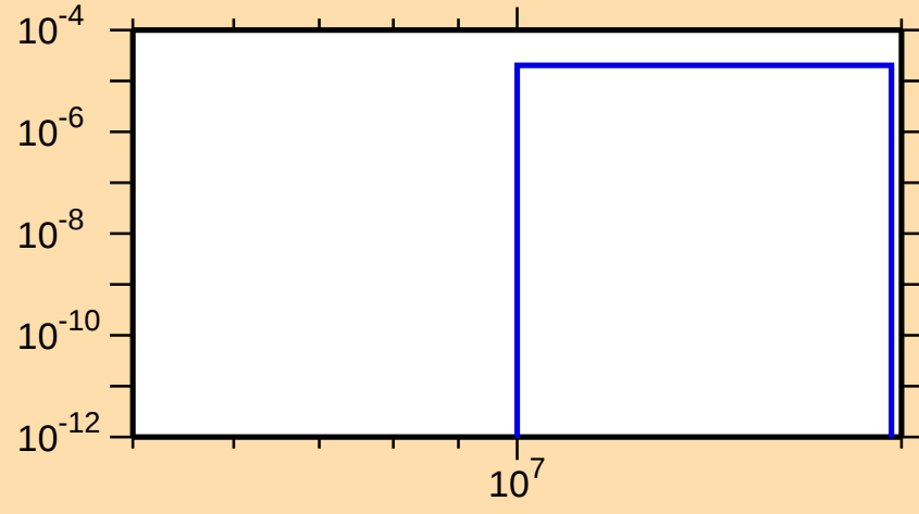
\sigma vs. E for ^{237}\text{Ac}(n,t)
