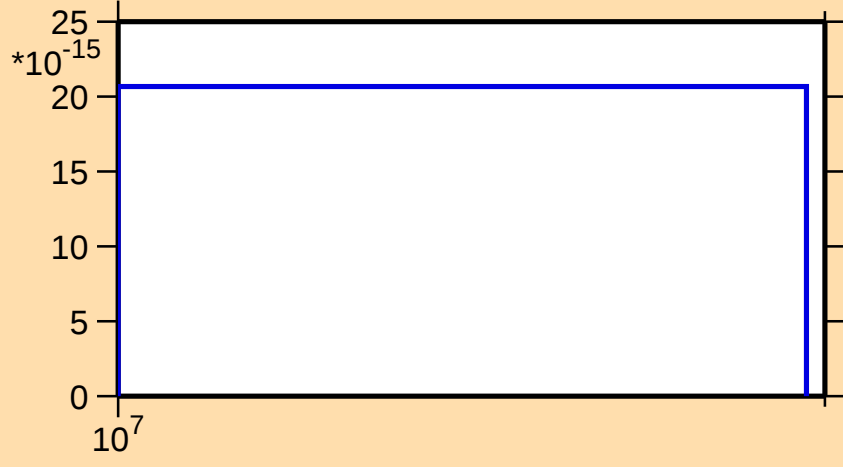
\sigma vs. E for ^{237}\text{Ac}(n,3n\alpha)
