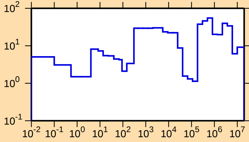
\Delta\sigma/\sigma vs. E for ^{237}\text{Ac}(n,\text{tot.})
