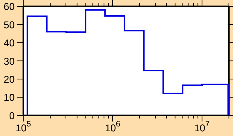
\Delta\sigma/\sigma vs. E for ^{237}\text{Ac}(\text{n},\text{inel.})
