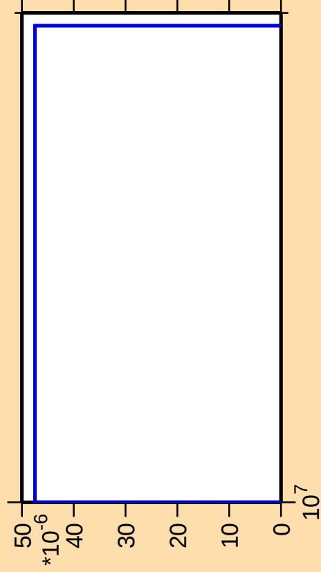
\Delta\sigma/\sigma vs. E for ^{237}\text{Ac}(\text{mt } 42)
