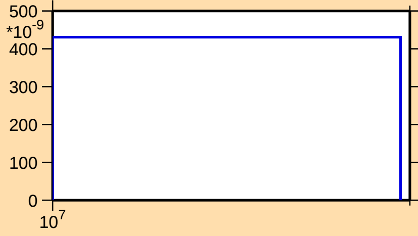
\sigma vs. E for ^{237}\text{Ac}(n,\text{nt})
