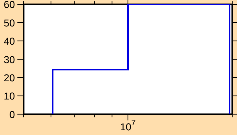
\Delta\sigma/\sigma vs. E for ^{237}\text{Ac}(n,\text{ncont.})
