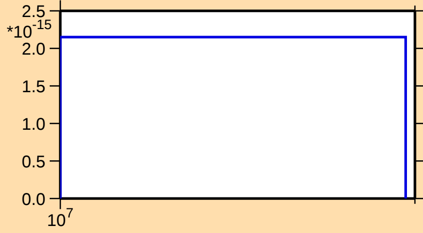
\sigma vs. E for ^{237}\text{Ac}(\text{mt } 42)
