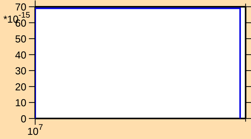
\sigma vs. E for ^{237}\text{Ac}(\text{mt } 11)
