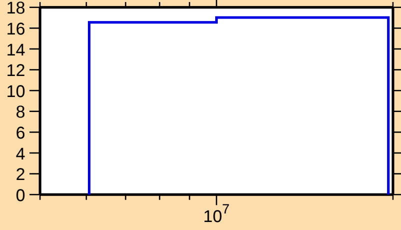
\Delta\sigma/\sigma vs. E for ^{237}\text{Ac}(n,\text{inel.})
