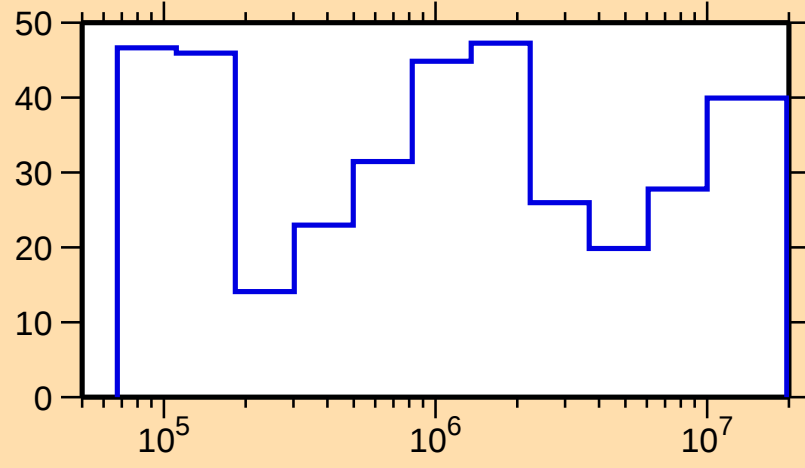
\Delta\sigma/\sigma vs. E for ^{237}\text{Ac}(n,\text{nonel.})
