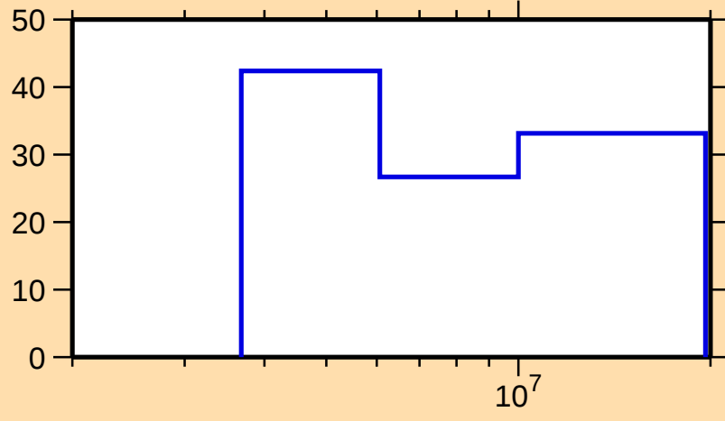
\Delta\sigma/\sigma vs. E for ^{237}\text{Ac}(n,2n)
