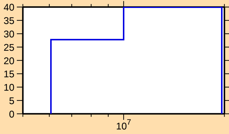
\Delta\sigma/\sigma vs. E for ^{237}\text{Ac}(n,\text{nonel.})
