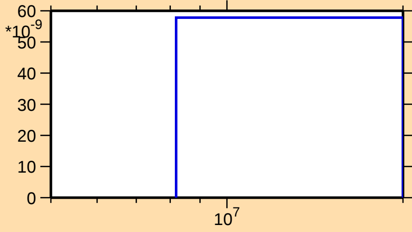
\sigma vs. E for ^{95}\text{Ag}(n,\text{pt})
