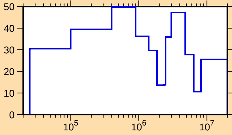
\Delta\sigma/\sigma vs. E for ^{95}\text{Ag}(n,\text{el.})
