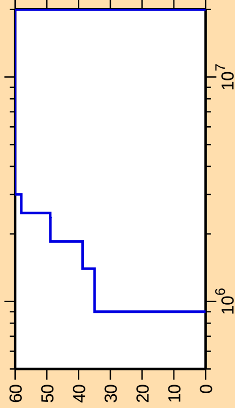
\Delta\sigma/\sigma vs. E for ^{95}\text{Ag}(n,p)
