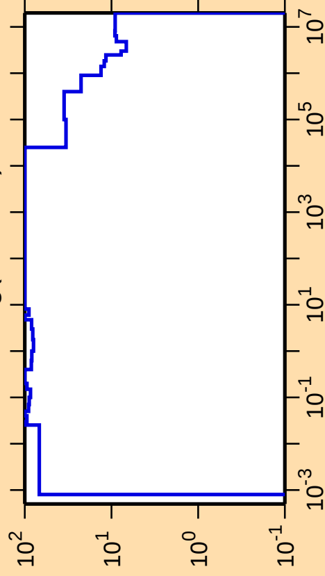
\Delta\sigma/\sigma vs. E for ^{95}\text{Ag}(n,\text{nonel.})
