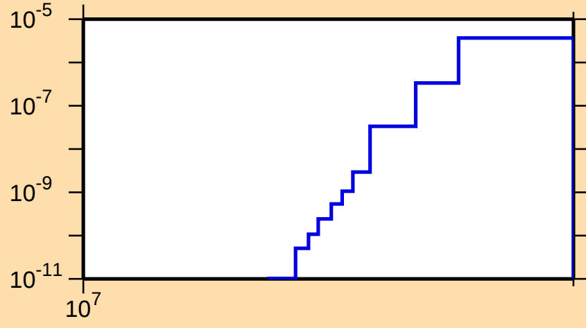
\sigma vs. E for ^{96}\text{Ag}(\text{mt } 45)
