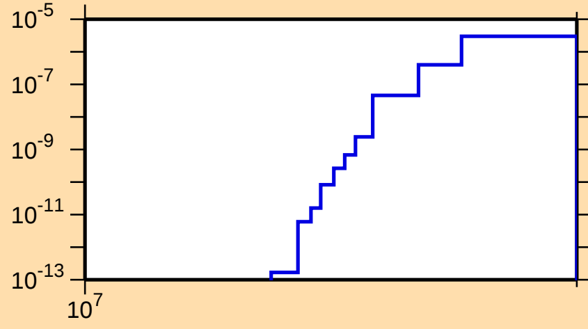
\sigma vs. E for ^{96}\text{Ag}(n,\text{nd})
