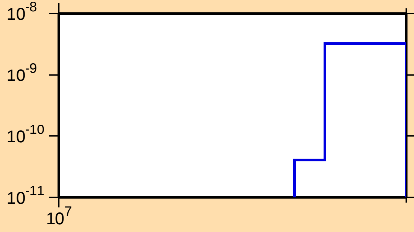
\sigma vs. E for ^{96}\text{Ag}(\text{mt } 34)
