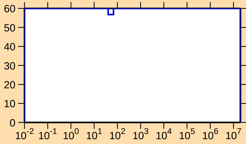
\Delta\sigma/\sigma vs. E for ^{96}\text{Ag}(n,\gamma)
