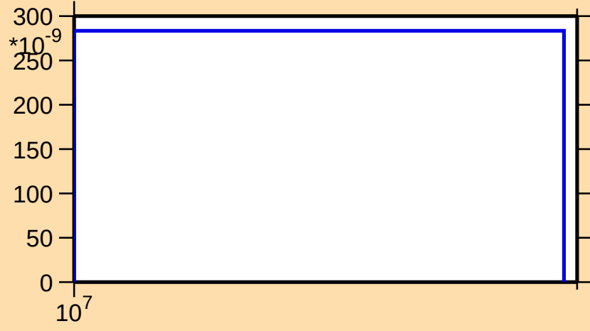
\sigma vs. E for ^{96}\text{Ag}(n,2np)
