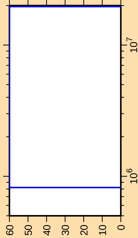
\Delta\sigma/\sigma vs. E for ^{96}\text{Ag}(n,d)
