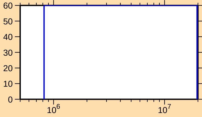
\Delta\sigma/\sigma vs. E for ^{96}\text{Ag}(n,n\text{cont.})
