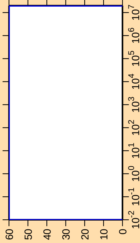
\Delta\sigma/\sigma vs. E for ^{96}\text{Ag}(n,\alpha)
