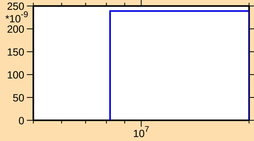
\sigma vs. E for ^{96}\text{Ag}(n,2np)
