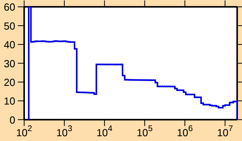
\Delta\sigma/\sigma vs. E for ^{101}\text{Ag}(n,\text{nonel.})
