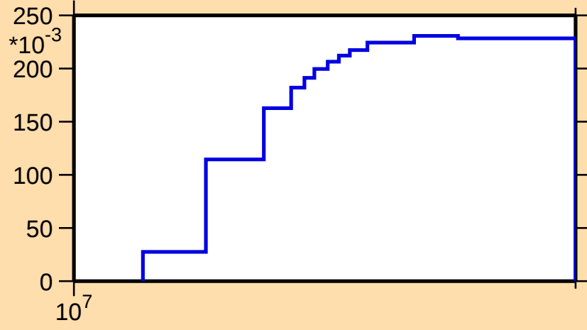
\sigma vs. E for ^{101}\text{Ag}(n,2n)
