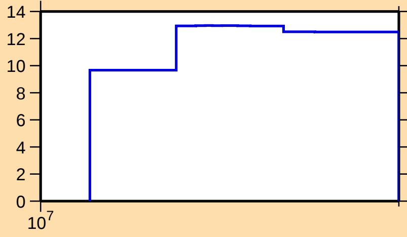
\Delta\sigma/\sigma vs. E for ^{101}\text{Ag}(n,\text{tot.})
