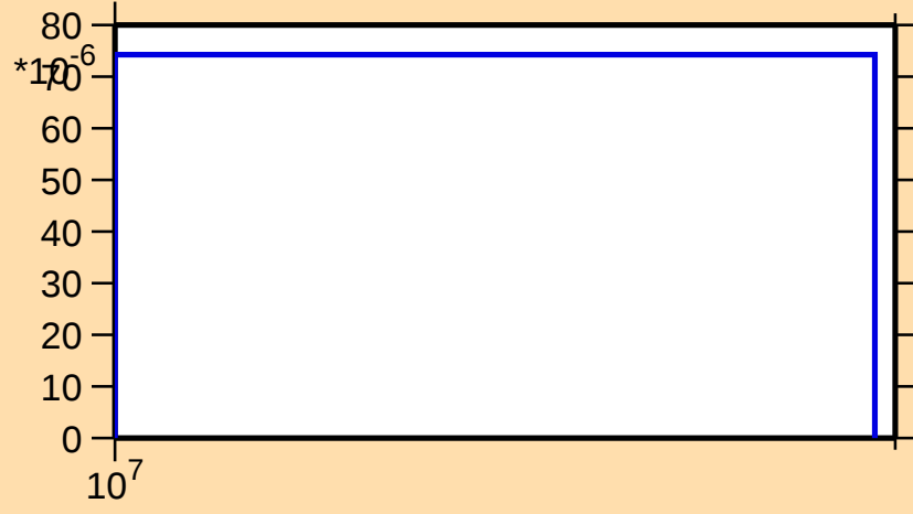
\sigma vs. E for ^{101}\text{Ag}(n,2np)
