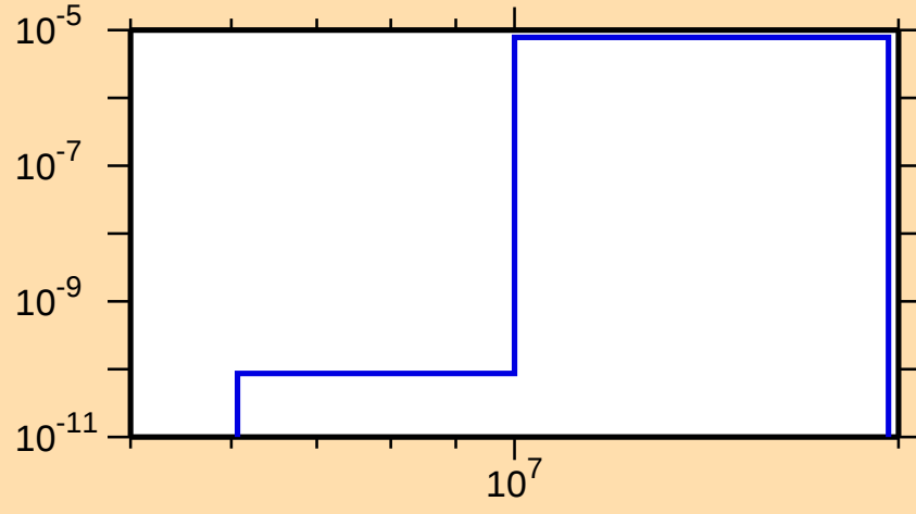
\sigma vs. E for ^{101}\text{Ag}(n,\text{He}3)
