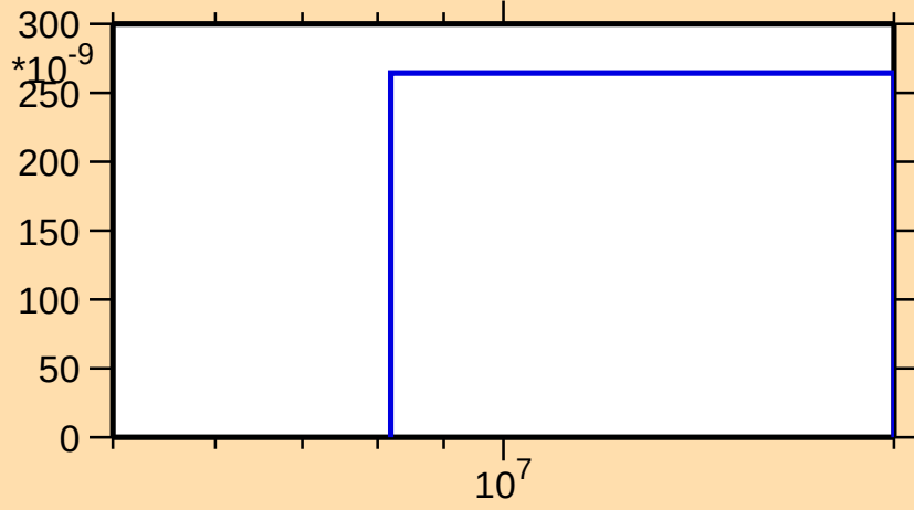
\sigma vs. E for ^{101}\text{Ag}(\text{mt117})
