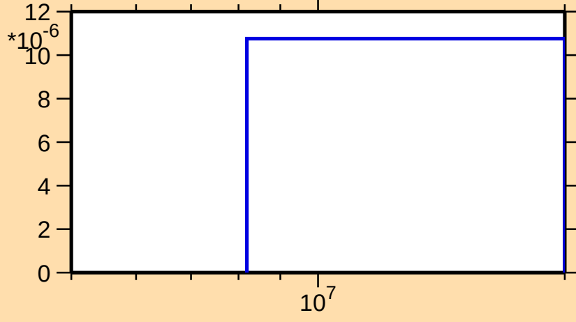
\sigma vs. E for ^{101}\text{Ag}(n,\text{pd})
