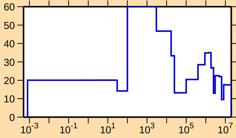
\Delta\sigma/\sigma vs. E for ^{101}\text{Ag}(n,\text{el.})
