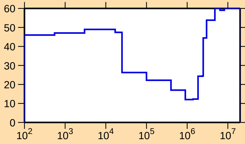
\Delta\sigma/\sigma vs. E for ^{101}\text{Ag}(n,n_1)
