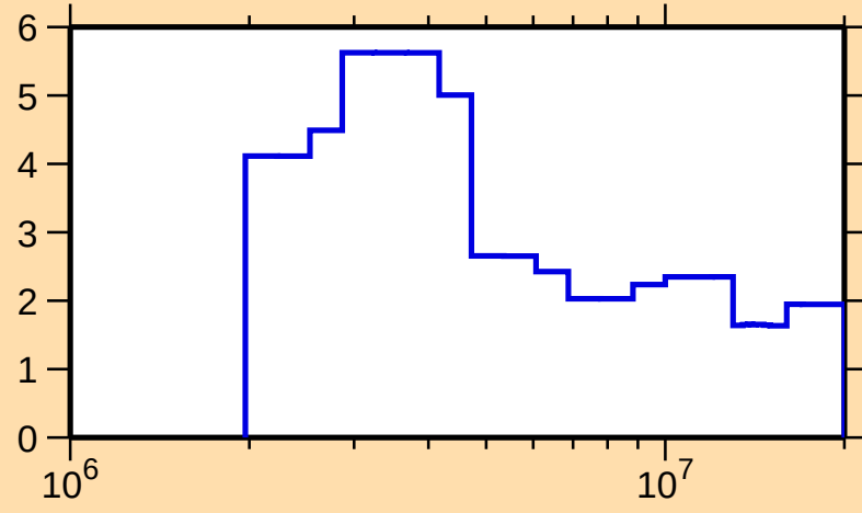
\Delta\sigma/\sigma vs. E for ^{102}\text{Ag}(n,n\text{onel.})
