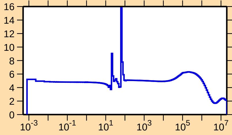
\sigma vs. E for ^{102}\text{Ag}(n,\text{el.})
