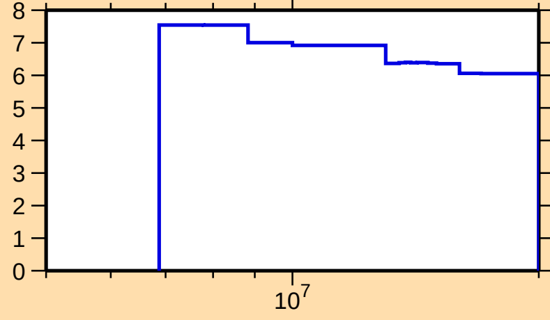
\Delta\sigma/\sigma vs. E for ^{108}\text{Ag}(n,\text{nonel.})
