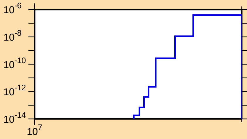
\sigma vs. E for ^{108}\text{Ag}(n,2n\alpha)
