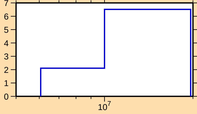
\Delta\sigma/\sigma vs. E for ^{108}\text{Ag}(n,\text{tot.})
