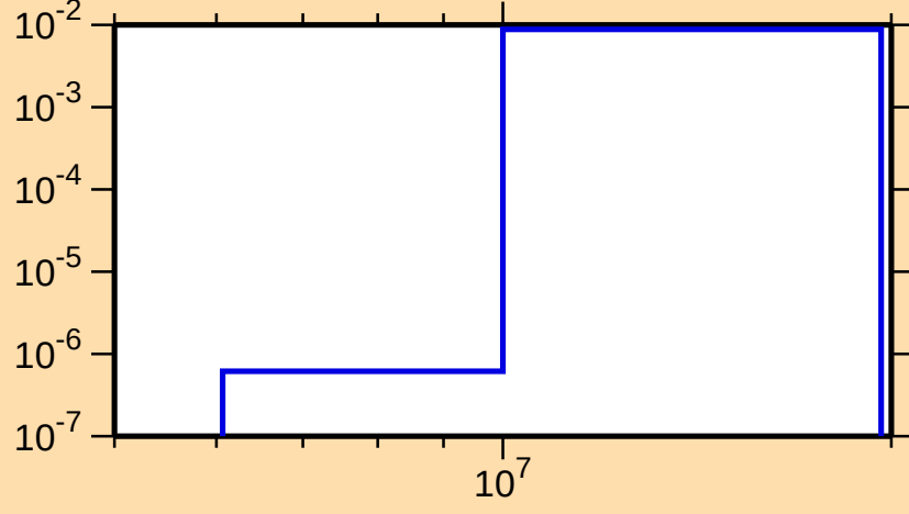
\sigma vs. E for ^{108}\text{Ag}(n,np)
