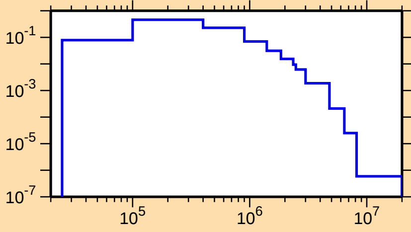
\sigma vs. E for ^{108}\text{Ag}(n,n_3)
