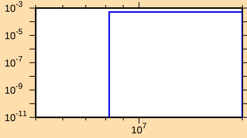
\sigma vs. E for ^{108}\text{Ag}(n,n\alpha)
