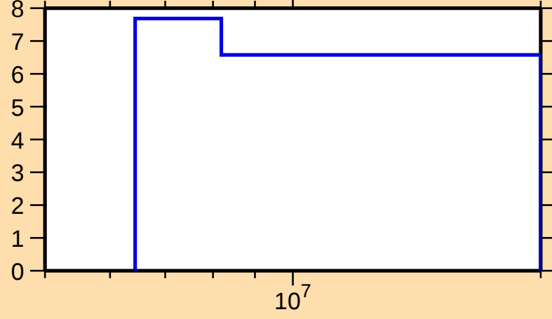
\Delta\sigma/\sigma vs. E for ^{108}\text{Ag}(n,\text{nonel.})
