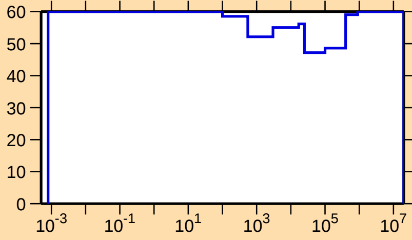
\Delta\sigma/\sigma vs. E for ^{108}\text{Ag}(n,p)
