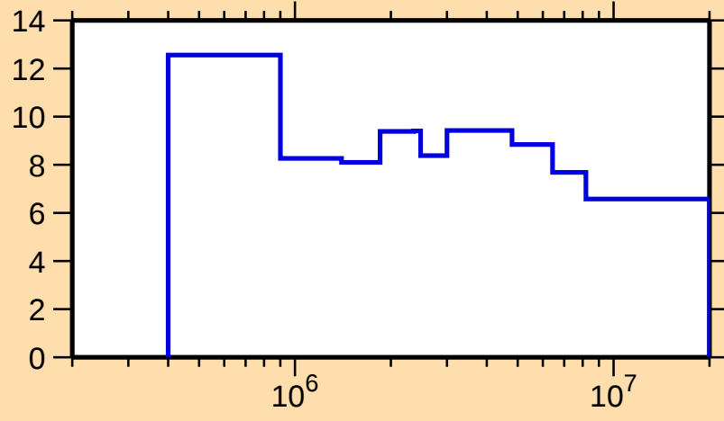
\Delta\sigma/\sigma vs. E for ^{108}\text{Ag}(n,n\text{onl.})
