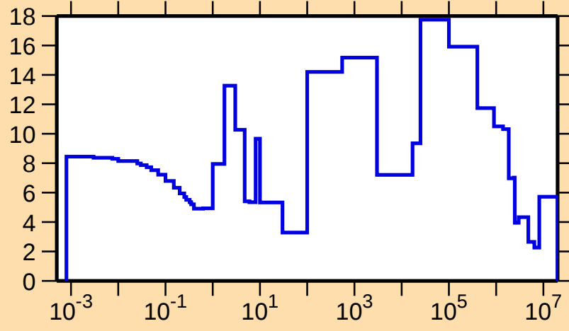
\Delta\sigma/\sigma vs. E for ^{108}\text{Ag}(n,\text{tot.})
