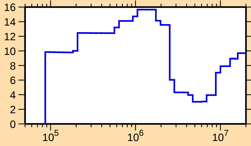
\Delta\sigma/\sigma vs. E for ^{109}\text{Ag}(n,\text{tot.})
