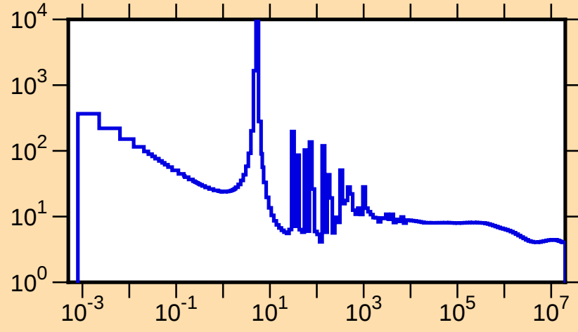
\sigma vs. E for ^{109}\text{Ag}(n,\text{tot.})
