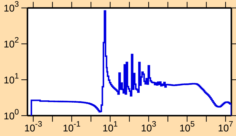
\sigma vs. E for ^{109}\text{Ag}(n,\text{el.})
