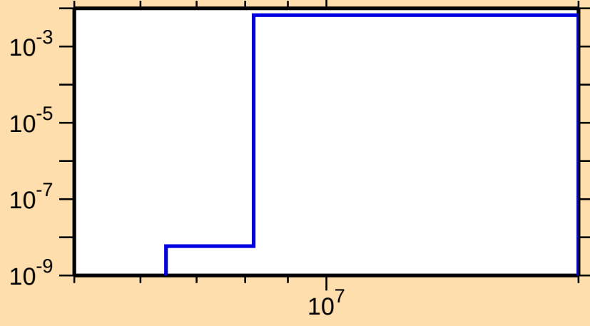
\sigma vs. E for ^{109}\text{Ag}(n,np)
