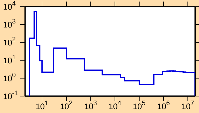
\sigma vs. E for ^{109}\text{Ag}(n,\text{nonel.})
