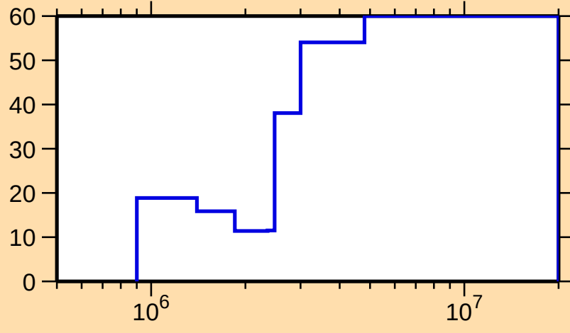
\Delta\sigma/\sigma vs. E for ^{109}\text{Ag}(n,n_1)
