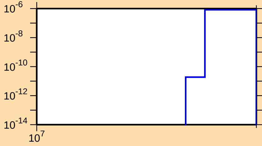
\sigma vs. E for ^{109}\text{Ag}(n,2np)
