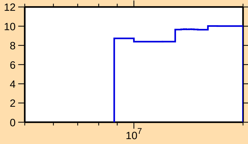
\Delta\sigma/\sigma vs. E for ^{109}\text{Ag}(n,\text{nonel.})
