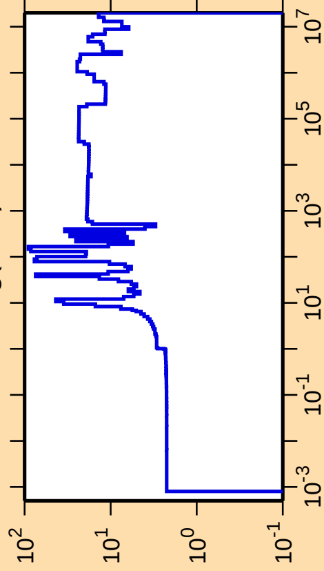
\Delta\sigma/\sigma vs. E for ^{111}\text{Ag}(n,\text{el.})
