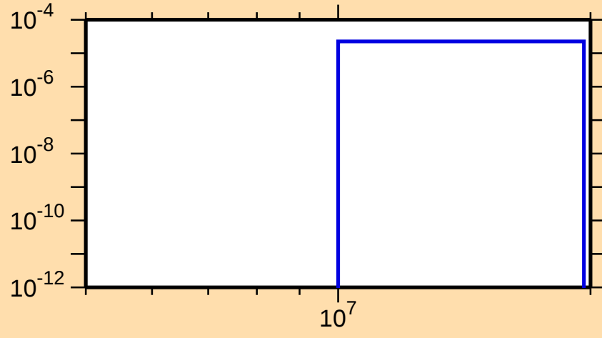
\sigma vs. E for ^{111}\text{Ag}(n,t)
