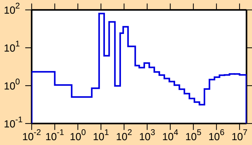
\sigma vs. E for ^{111}\text{Ag}(n,\text{nonel.})
