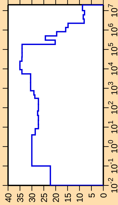
\Delta\sigma/\sigma vs. E for ^{111}\text{Ag}(n,\text{nonel.})
