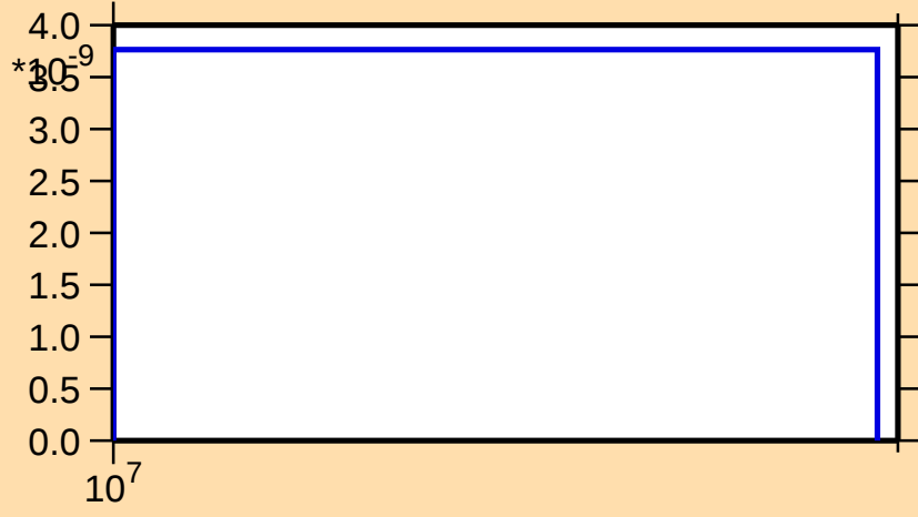
\sigma vs. E for ^{111}\text{Ag}(n,2np)
