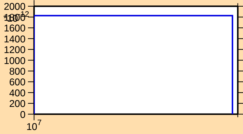
\sigma vs. E for ^{111}\text{Ag}(n,\text{nt})
