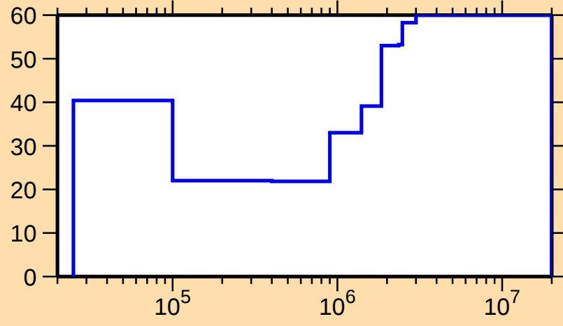
\Delta\sigma/\sigma vs. E for ^{111}\text{Ag}(n,n_1)
