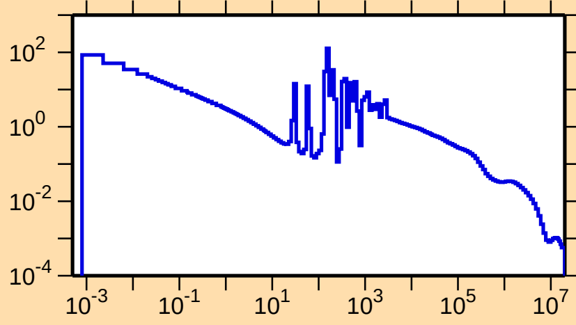
\sigma vs. E for ^{113}\text{Ag}(n,\gamma)
