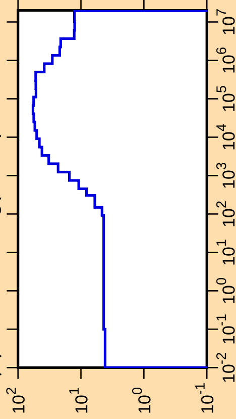
\Delta\mu/\mu vs. E for ^{113}\text{Ag}(\text{mt251})
