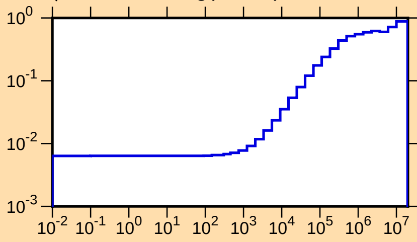
\mu vs. E for ^{113}\text{Ag}(\text{mt251})
