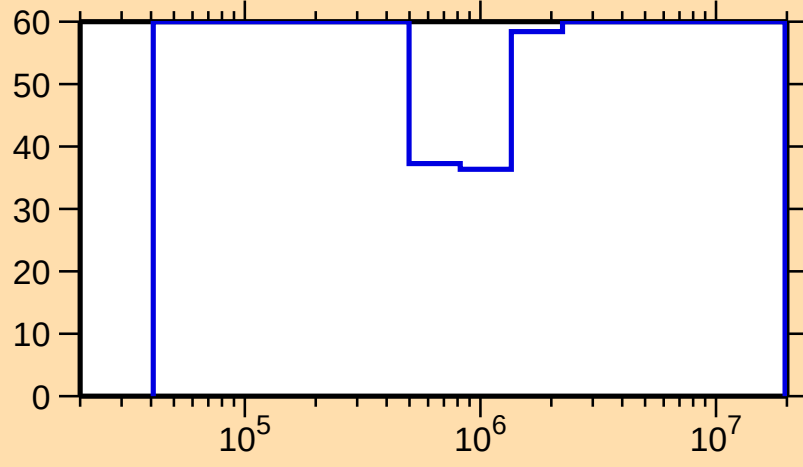
\Delta\sigma/\sigma vs. E for ^{113}\text{Ag}(n,n_1)
