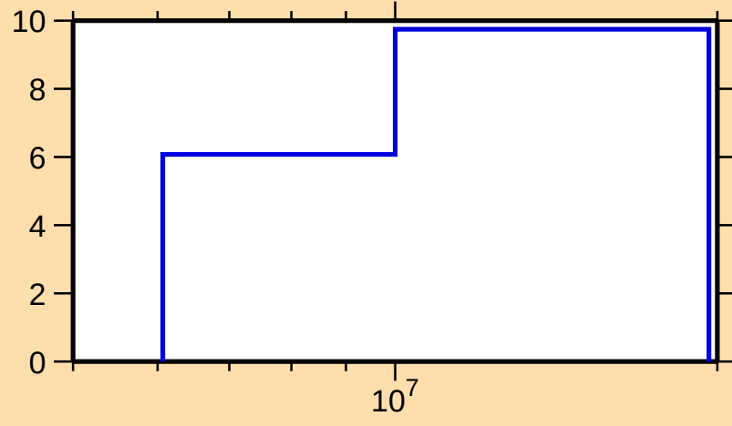
\Delta\sigma/\sigma vs. E for ^{113}\text{Ag}(n,\text{tot.})
