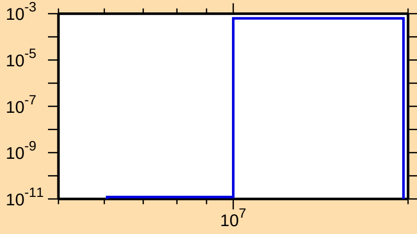
\sigma vs. E for ^{113}\text{Ag}(n,np)
