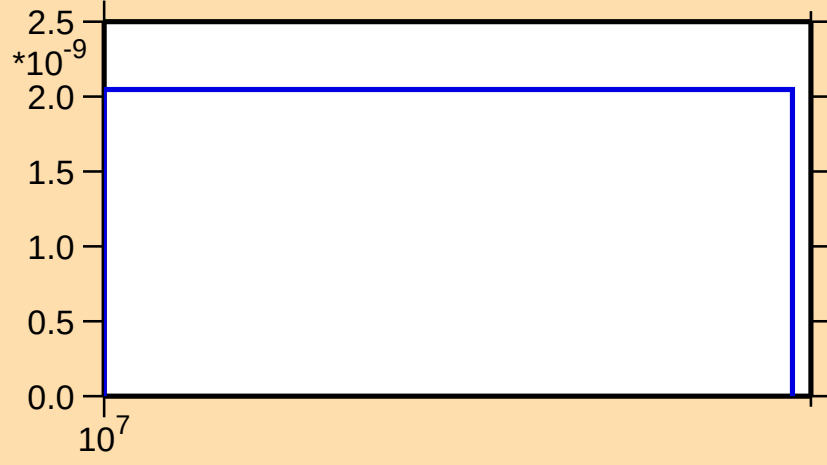
\sigma vs. E for ^{113}\text{Ag}(n,nt)
