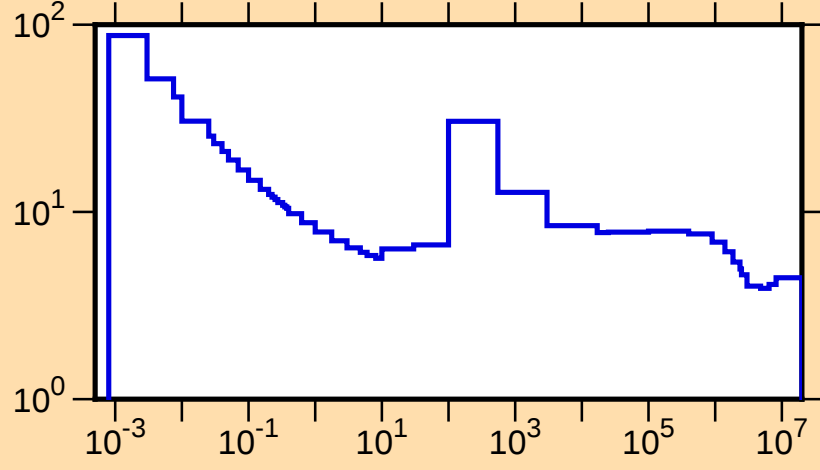
\sigma vs. E for ^{113}\text{Ag}(n,\text{tot.})
