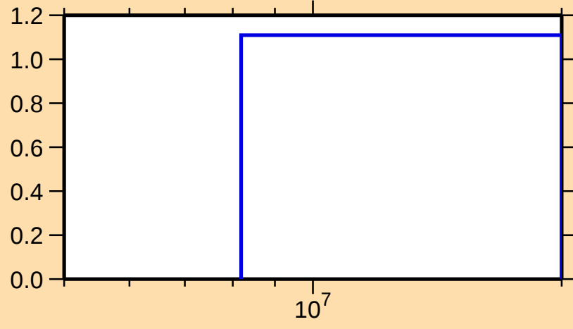
\sigma vs. E for ^{113}\text{Ag}(n,2n)
