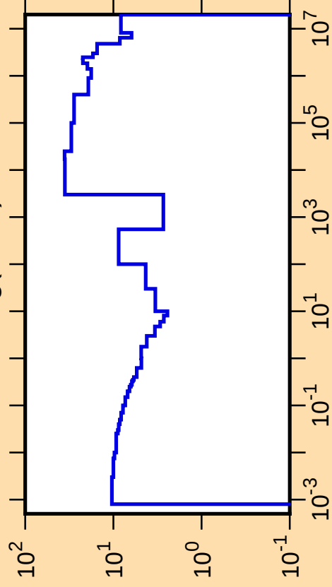
\Delta\sigma/\sigma vs. E for ^{113}\text{Ag}(n,\text{tot.})
