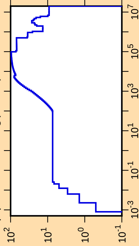
\Delta\mu/\mu vs. E for ^{115}\text{Ag}(\text{mt251})
