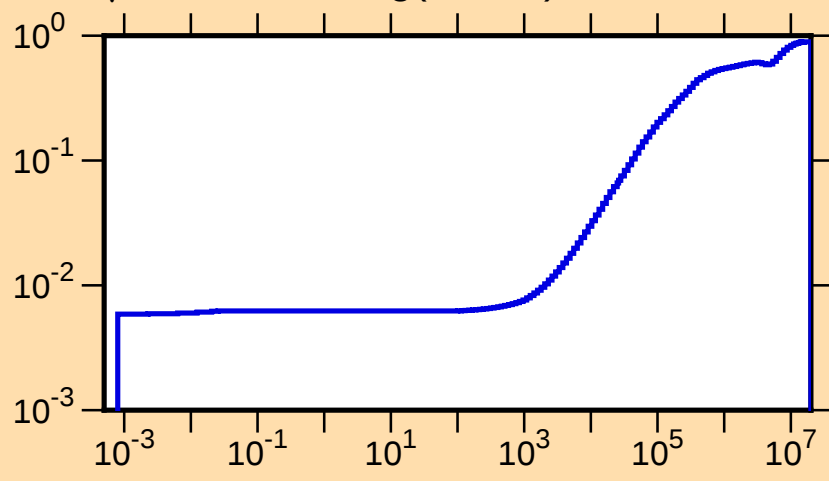
\mu vs. E for ^{115}\text{Ag}(\text{mt251})
