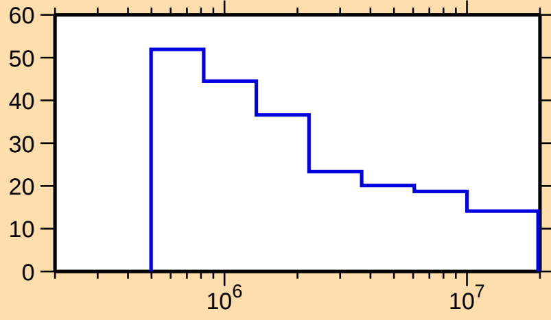
\Delta\sigma/\sigma vs. E for ^{115}\text{Ag}(n,n\text{onel.})
