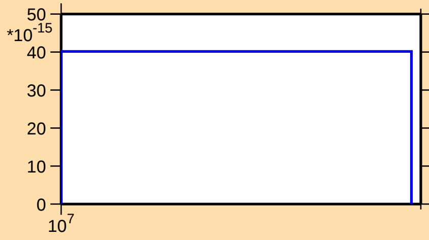
\sigma vs. E for ^{115}\text{Ag}(n,2n\alpha)
