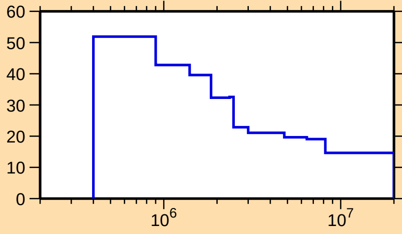
\Delta\sigma/\sigma vs. E for ^{115}\text{Ag}(n,\text{nonel.})
