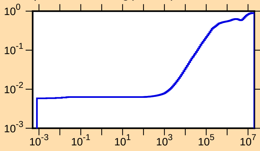
\mu vs. E for ^{116}\text{Ag}(\text{mt251})
