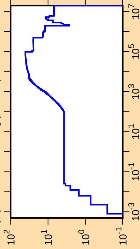
\Delta\mu/\mu vs. E for ^{116}\text{Ag}(\text{mt251})
