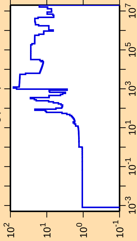
\Delta\sigma/\sigma vs. E for ^{116}\text{Ag}(n,\text{el.})
